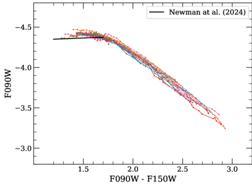
Figure 11. from Maksim I. Chazov et al 2026 Astrophys. J. 1001 doi:10.3847/1538-4357/ae50ed https://dx.doi.org/10.3847/1538-4357/ae50ed © 2026. The Author(s). Published by the American Astronomical Society.
