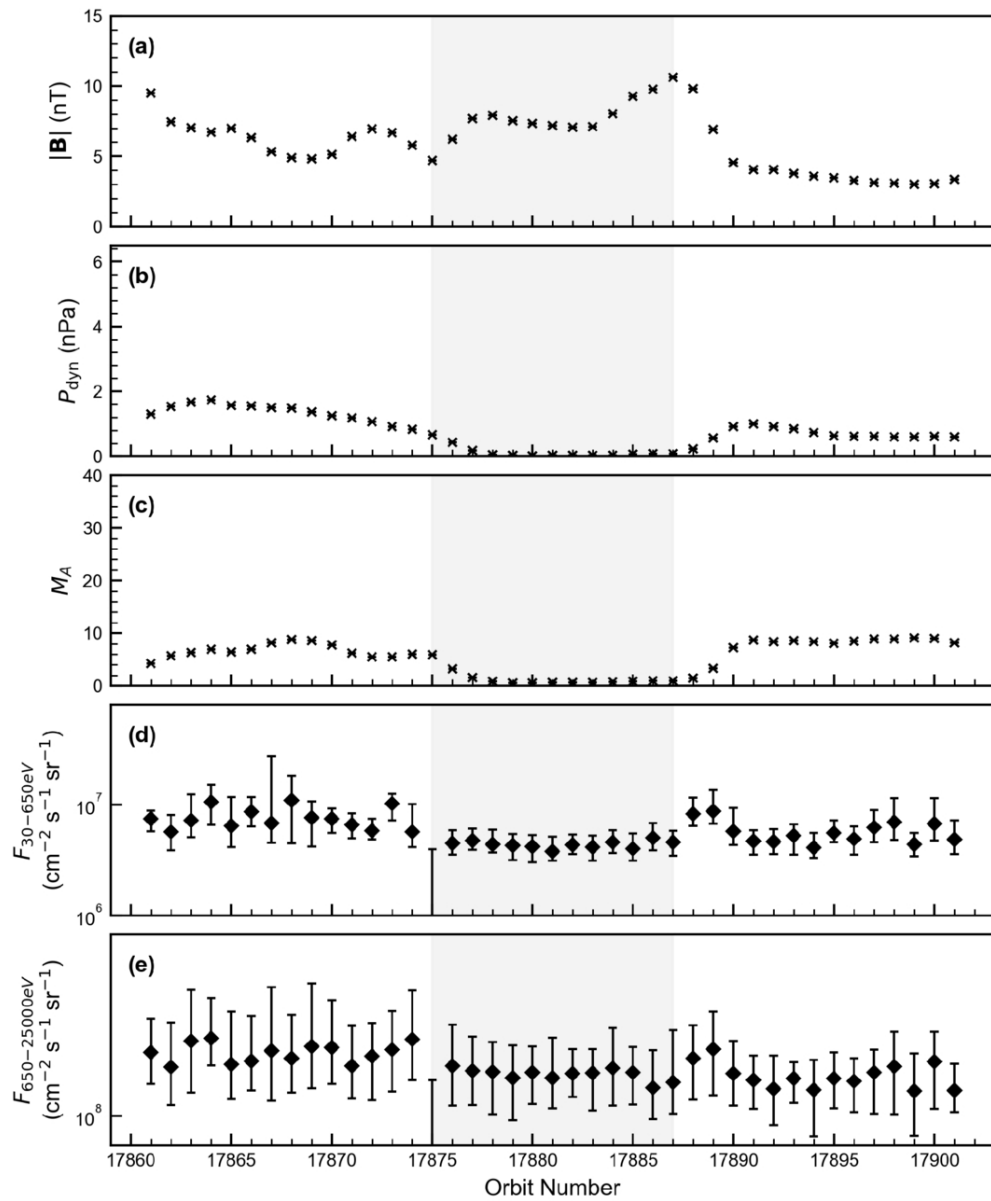
Figure 9. from Xinzhi Qiu et al 2026 Astrophys. J. 1001 doi:10.3847/1538-4357/ae5063 https://dx.doi.org/10.3847/1538-4357/ae5063 © 2026. The Author(s). Published by the American Astronomical Society.
