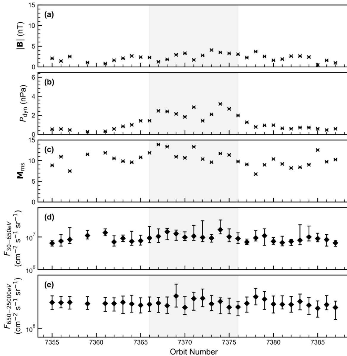
Figure 6. from Xinzhi Qiu et al 2026 Astrophys. J. 1001 doi:10.3847/1538-4357/ae5063 https://dx.doi.org/10.3847/1538-4357/ae5063 © 2026. The Author(s). Published by the American Astronomical Society.
