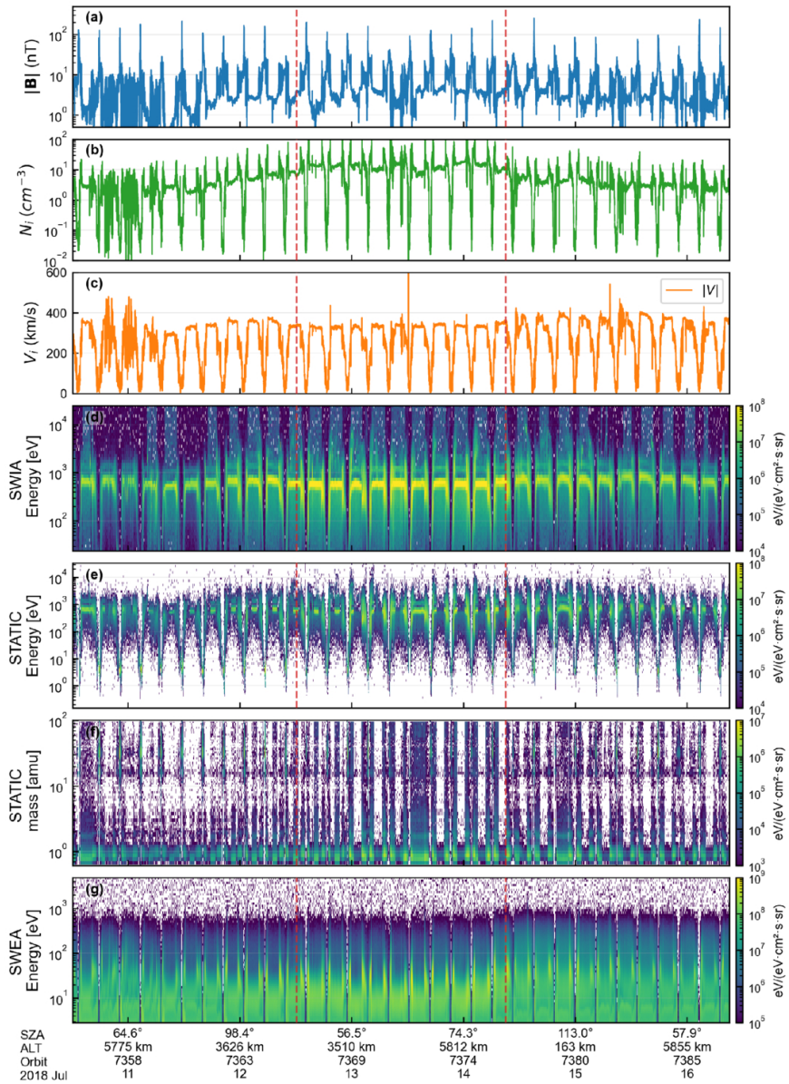
Figure 5. from Xinzhi Qiu et al 2026 Astrophys. J. 1001 doi:10.3847/1538-4357/ae5063 https://dx.doi.org/10.3847/1538-4357/ae5063 © 2026. The Author(s). Published by the American Astronomical Society.
