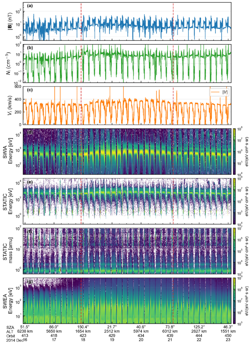
Figure 1. from Xinzhi Qiu et al 2026 Astrophys. J. 1001 doi:10.3847/1538-4357/ae5063 https://dx.doi.org/10.3847/1538-4357/ae5063 © 2026. The Author(s). Published by the American Astronomical Society.
