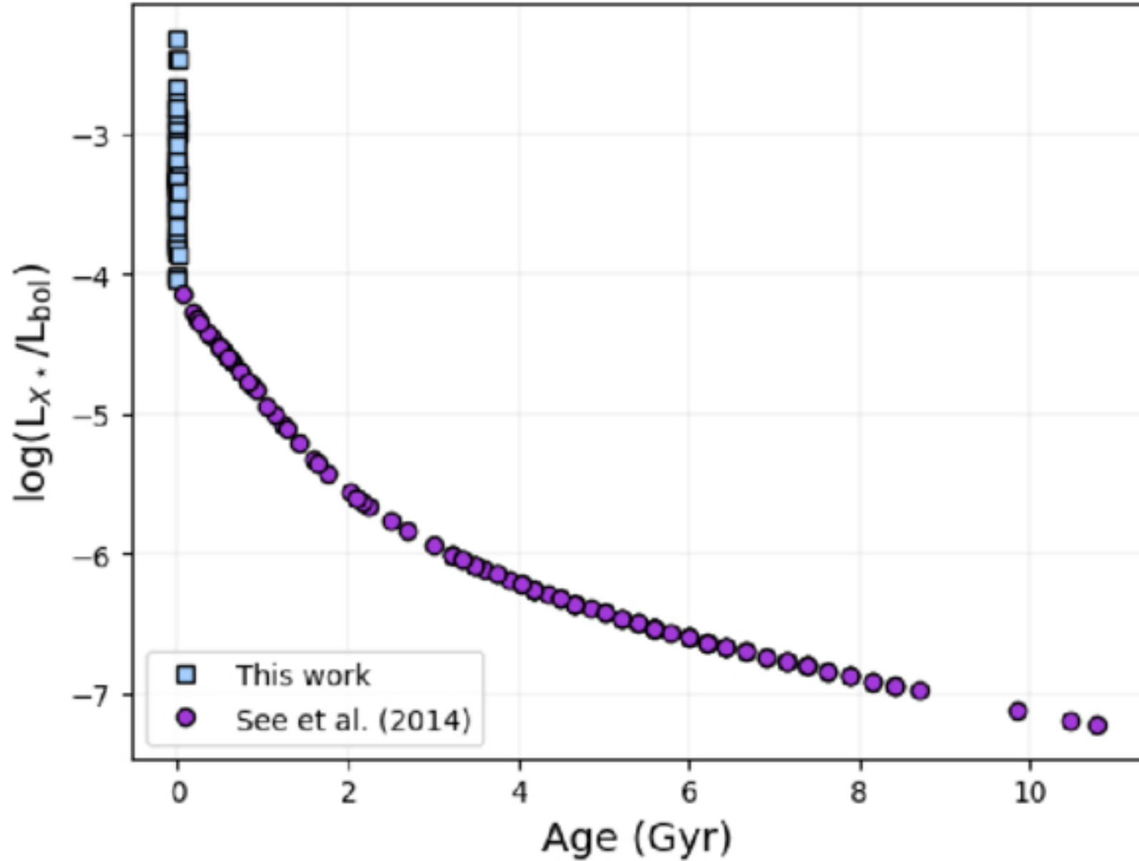
Figure 1. from Yasmin F. Tamburus et al 2026 Astrophys. J. 1001 doi:10.3847/1538-4357/ae5054 https://dx.doi.org/10.3847/1538-4357/ae5054 © 2026. The Author(s). Published by the American Astronomical Society.
