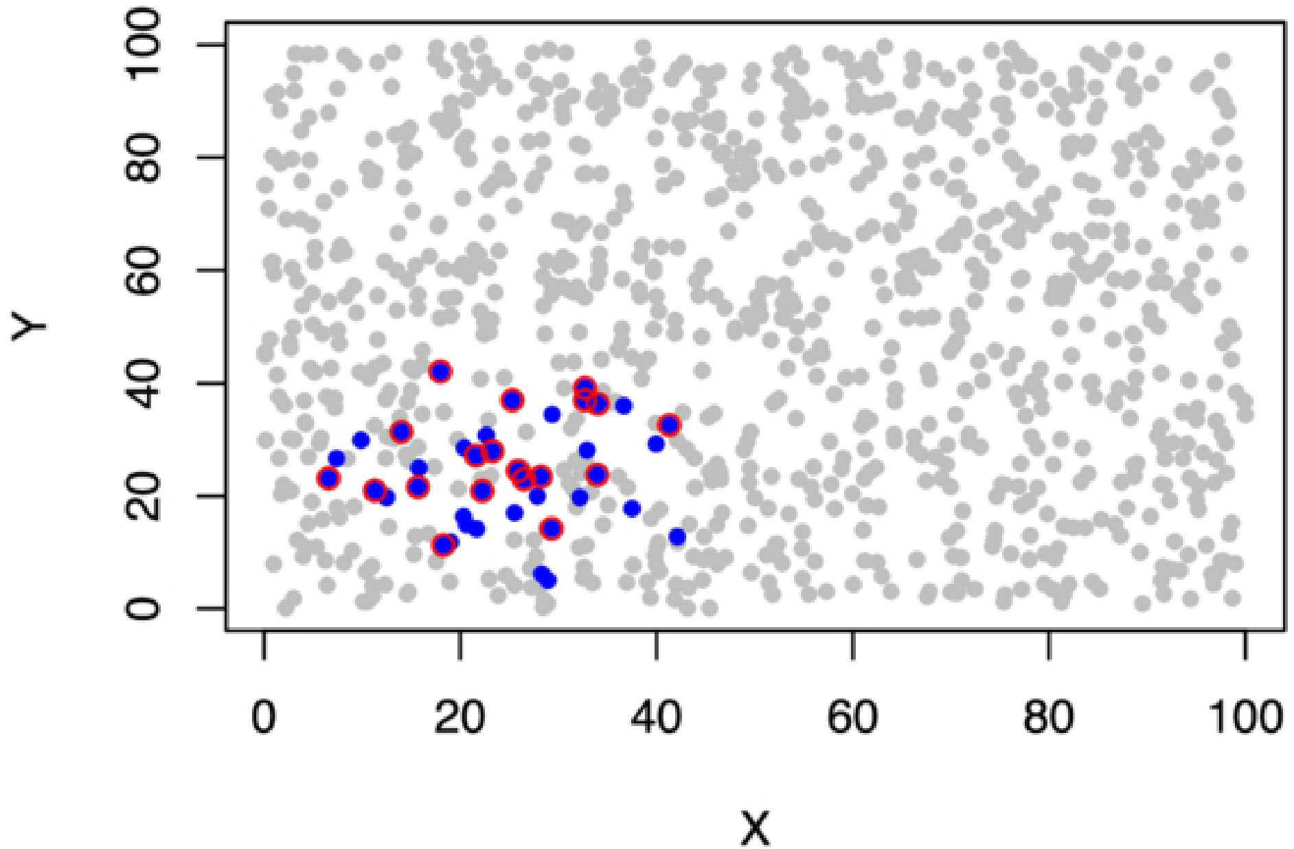
Figure 5. from Harrison B. Smith and Lana Sinapayen 2026 Astrophys. J. 1001 doi:10.3847/1538-4357/ae4ee3 https://dx.doi.org/10.3847/1538-4357/ae4ee3 © 2026. The Author(s). Published by the American Astronomical Society.
