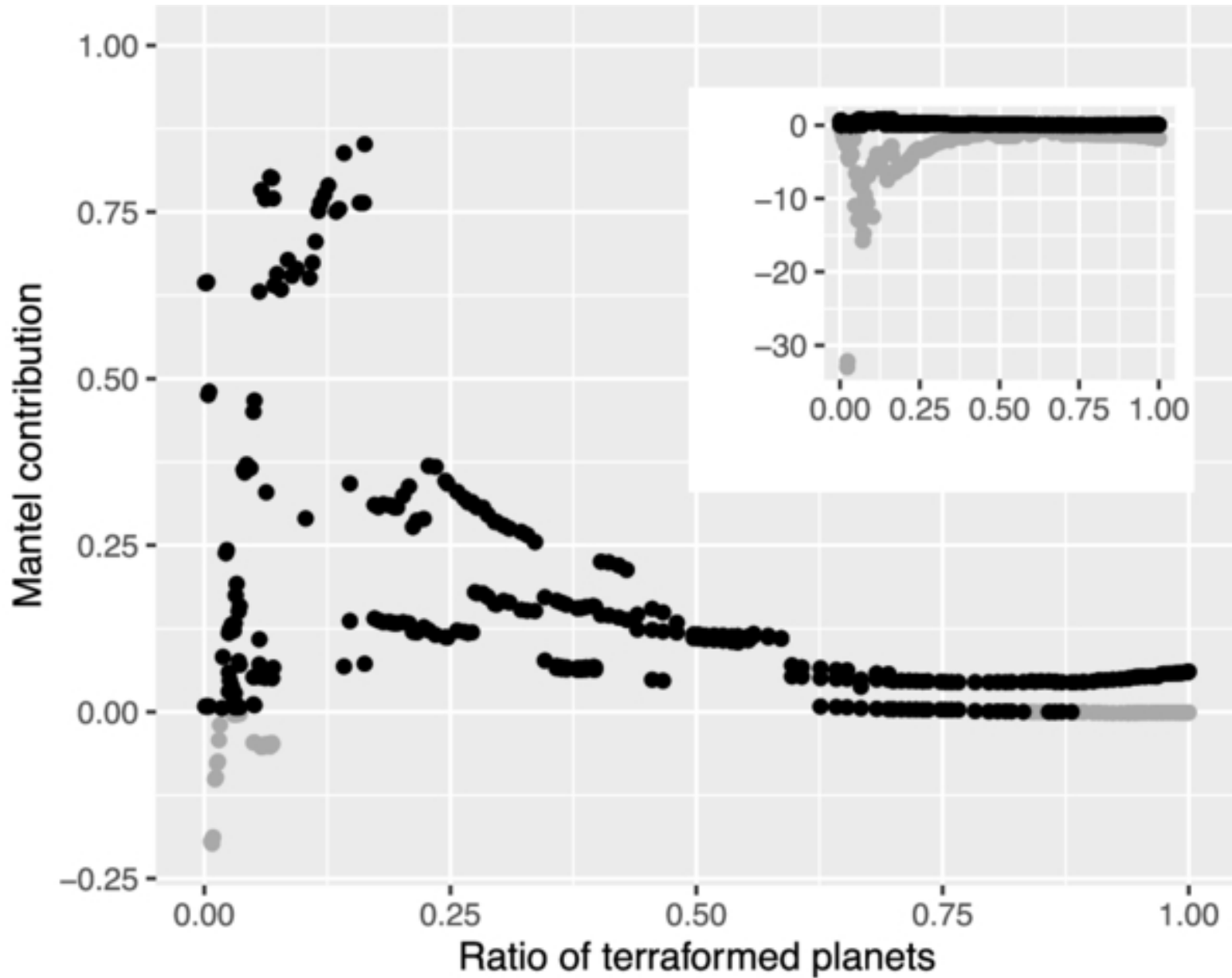
Figure 3. from Harrison B. Smith and Lana Sinapayen 2026 Astrophys. J. 1001 doi:10.3847/1538-4357/ae4ee3 https://dx.doi.org/10.3847/1538-4357/ae4ee3 © 2026. The Author(s). Published by the American Astronomical Society.
