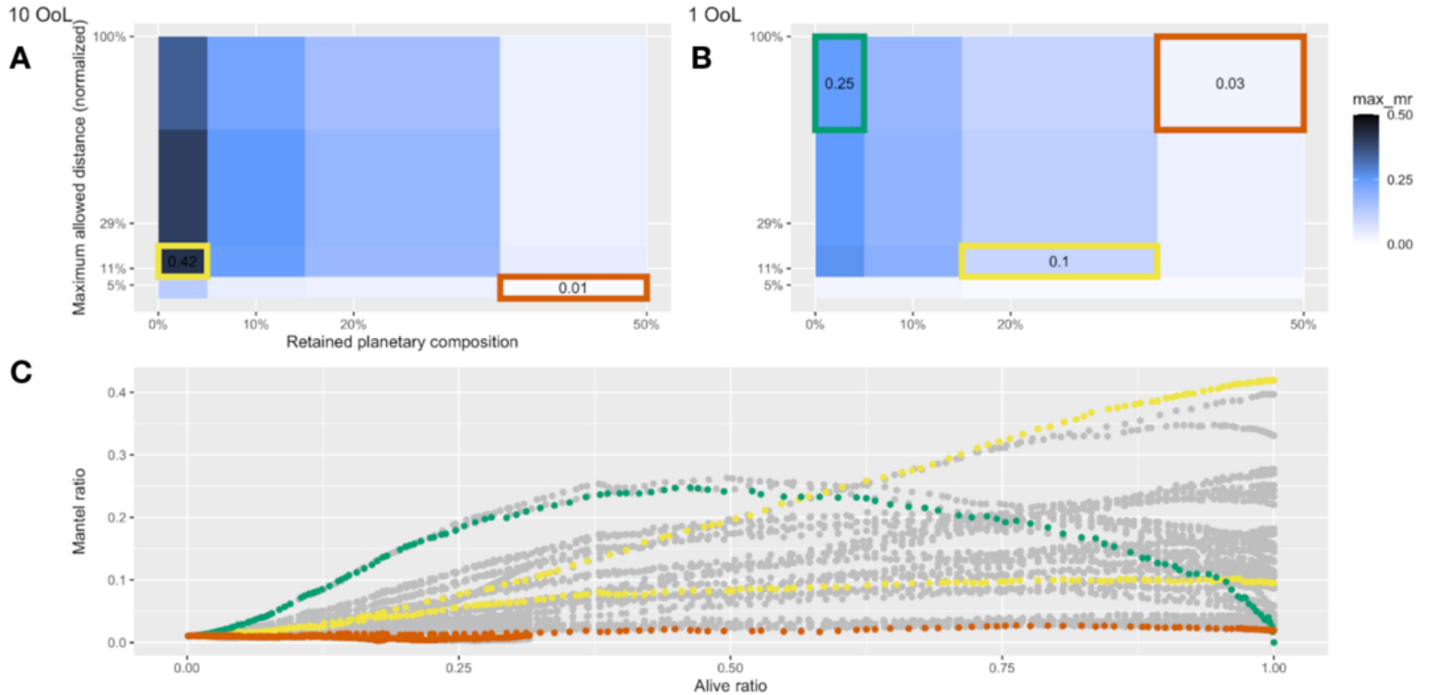
Figure A2. from Harrison B. Smith and Lana Sinapayen 2026 Astrophys. J. 1001 doi:10.3847/1538-4357/ae4ee3 https://dx.doi.org/10.3847/1538-4357/ae4ee3 © 2026. The Author(s). Published by the American Astronomical Society.
