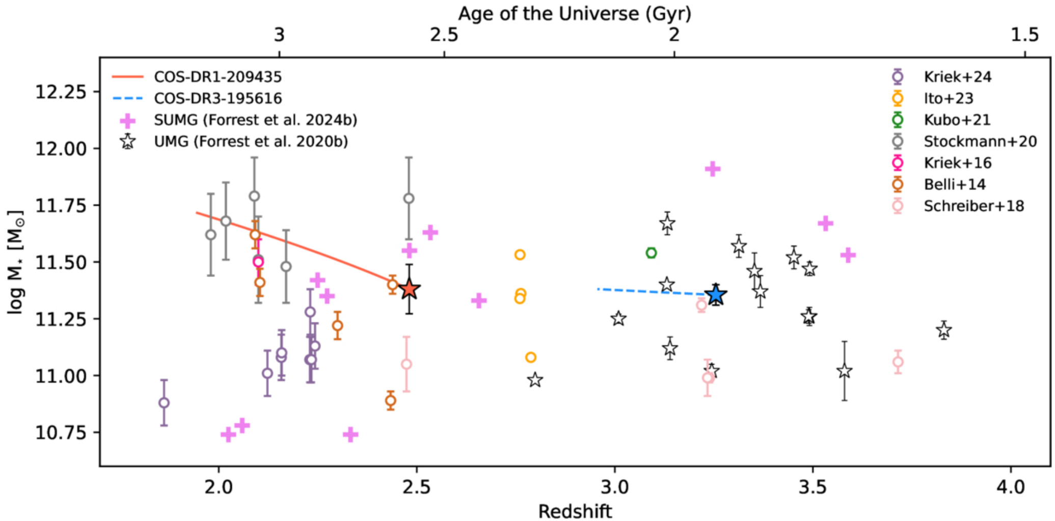
Figure 7. from Wenjun Chang et al 2026 Astrophys. J. 1001 doi:10.3847/1538-4357/ae4ede https://dx.doi.org/10.3847/1538-4357/ae4ede © 2026. The Author(s). Published by the American Astronomical Society.
