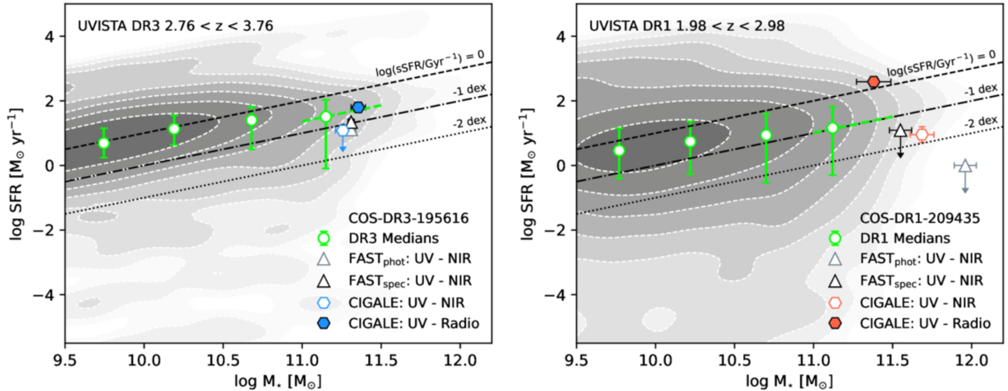
Figure 4. from Wenjun Chang et al 2026 Astrophys. J. 1001 doi:10.3847/1538-4357/ae4ede https://dx.doi.org/10.3847/1538-4357/ae4ede © 2026. The Author(s). Published by the American Astronomical Society.
