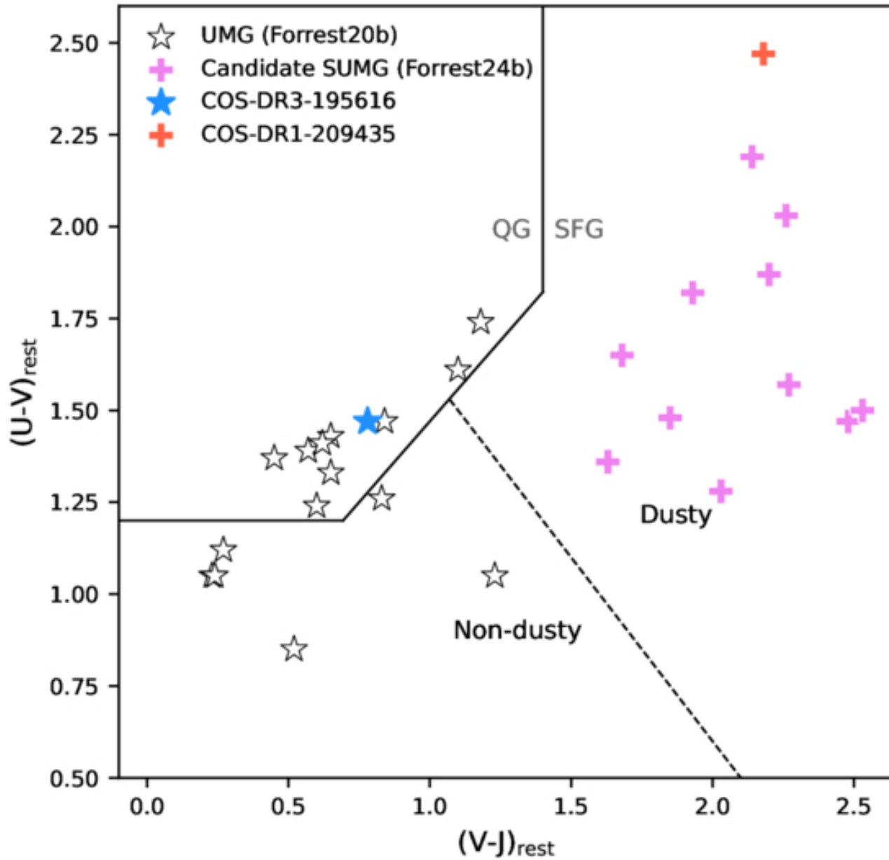
Figure 1. from Wenjun Chang et al 2026 Astrophys. J. 1001 doi:10.3847/1538-4357/ae4ede https://dx.doi.org/10.3847/1538-4357/ae4ede © 2026. The Author(s). Published by the American Astronomical Society.
