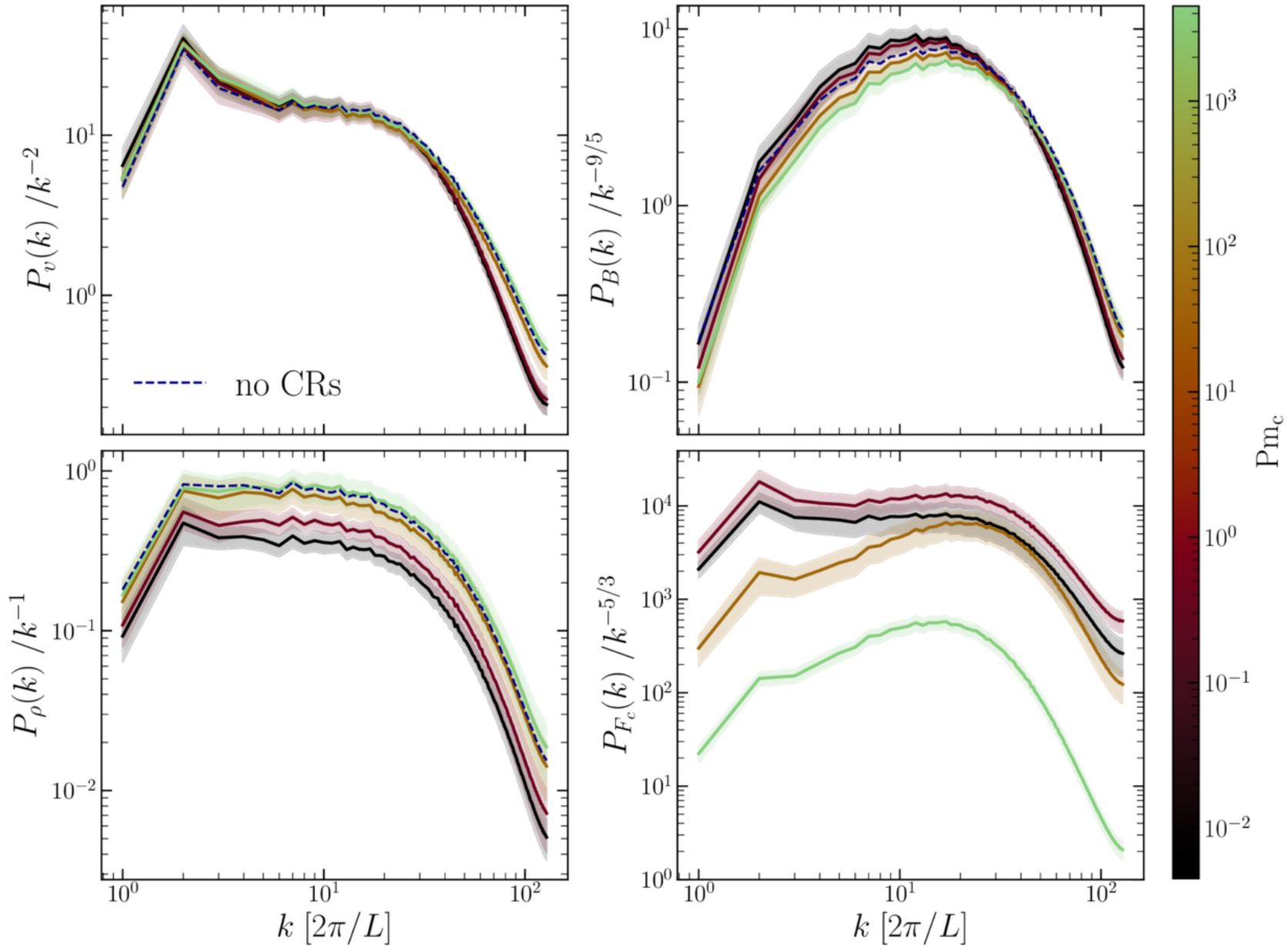
Figure 7. from Matt L. Sampson et al 2026 Astrophys. J. 1001 doi:10.3847/1538-4357/ae4edc https://dx.doi.org/10.3847/1538-4357/ae4edc © 2026. The Author(s). Published by the American Astronomical Society.
