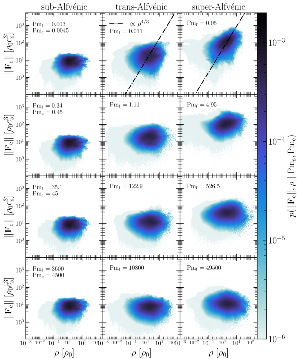
Figure 6. from Matt L. Sampson et al 2026 Astrophys. J. 1001 doi:10.3847/1538-4357/ae4edc https://dx.doi.org/10.3847/1538-4357/ae4edc © 2026. The Author(s). Published by the American Astronomical Society.
