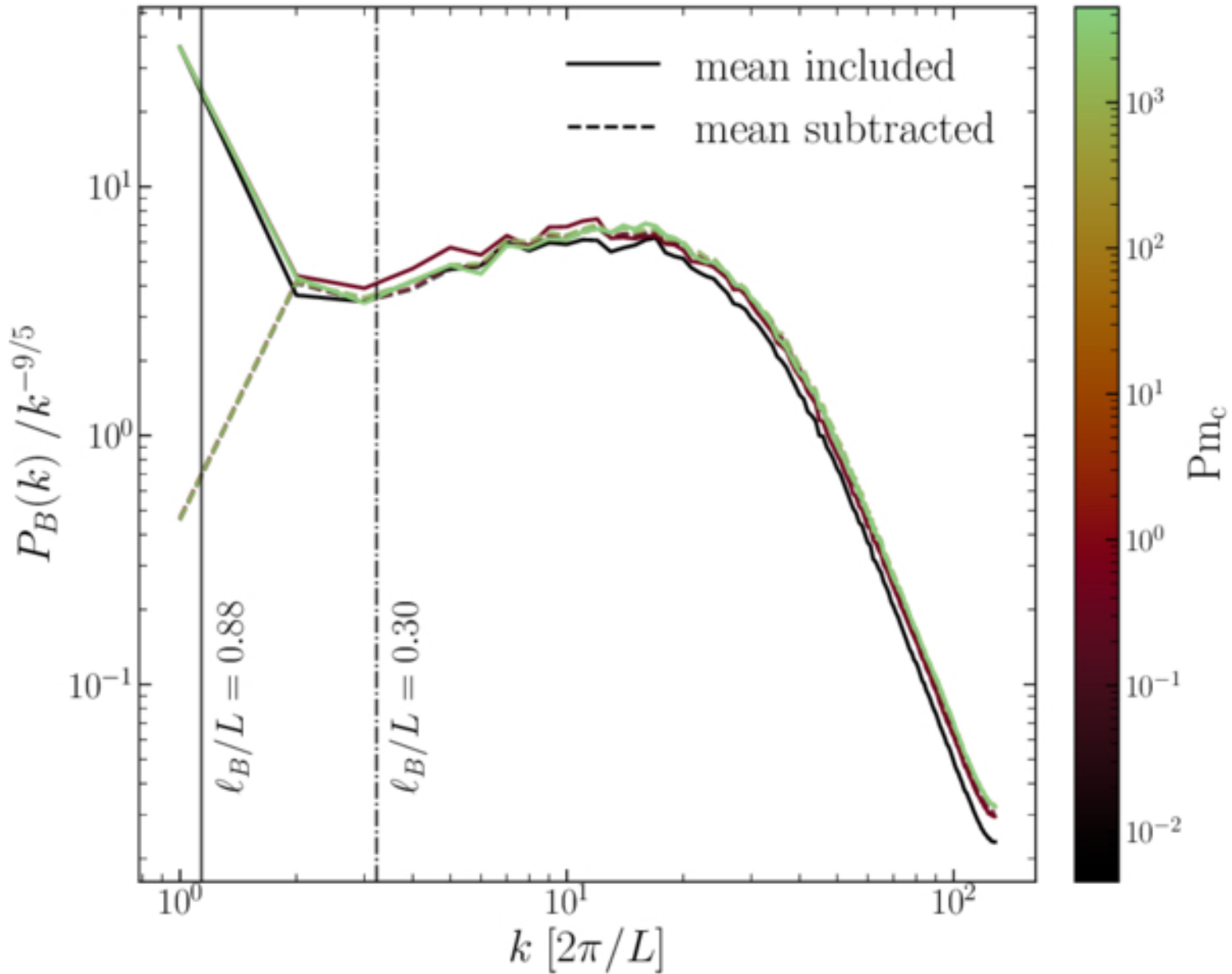
Figure 13. from Matt L. Sampson et al 2026 Astrophys. J. 1001 doi:10.3847/1538-4357/ae4edc https://dx.doi.org/10.3847/1538-4357/ae4edc © 2026. The Author(s). Published by the American Astronomical Society.
