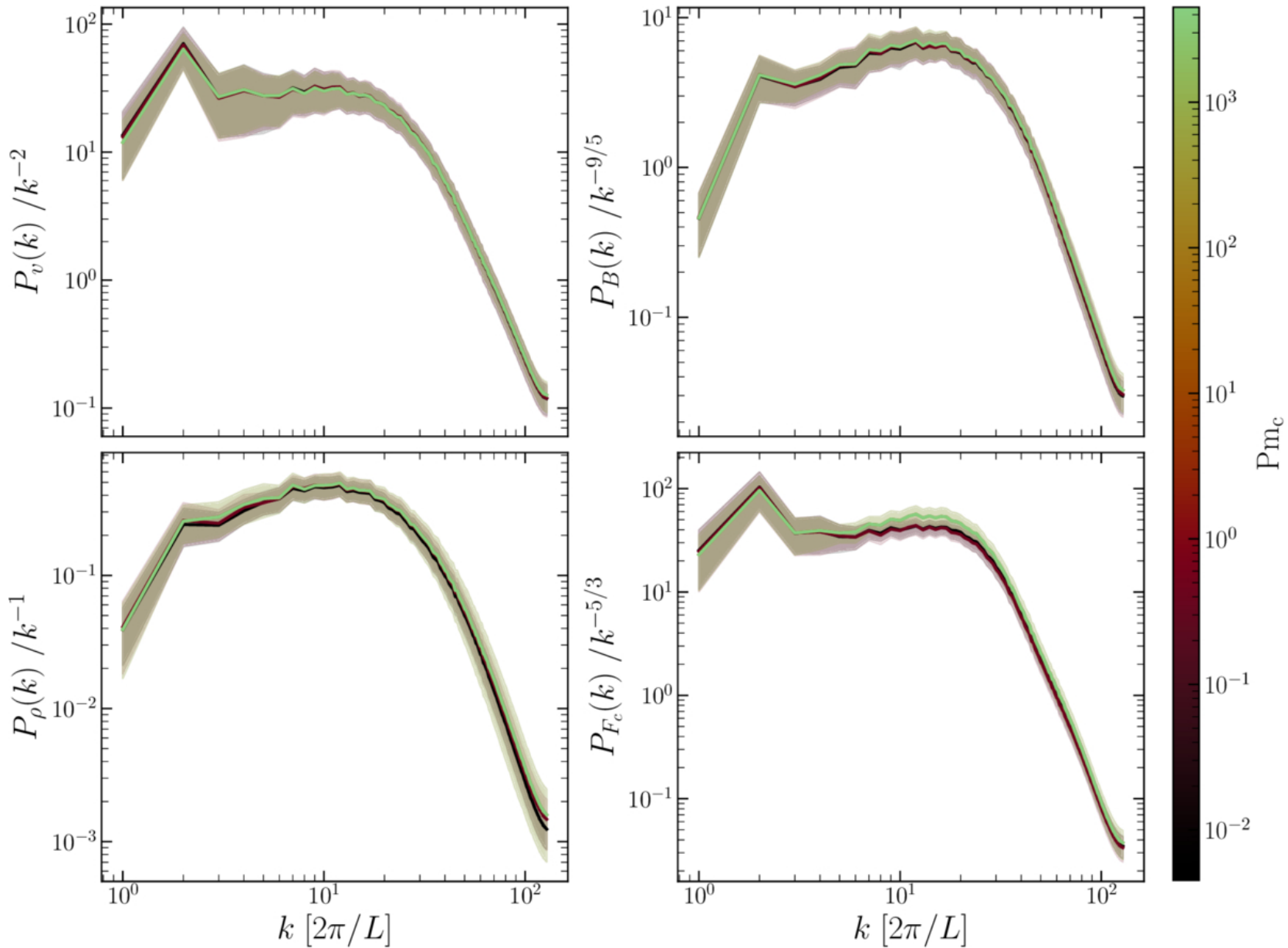
Figure 12. from Matt L. Sampson et al 2026 Astrophys. J. 1001 doi:10.3847/1538-4357/ae4edc https://dx.doi.org/10.3847/1538-4357/ae4edc © 2026. The Author(s). Published by the American Astronomical Society.
