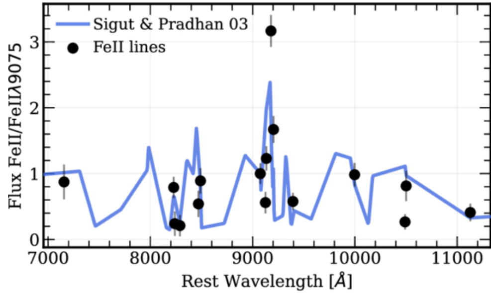
Figure 8. from Vasily Kokorev et al 2026 Astrophys. J. 1004 doi:10.3847/1538-4357/ae4ed7 https://dx.doi.org/10.3847/1538-4357/ae4ed7 © 2026. The Author(s). Published by the American Astronomical Society.
