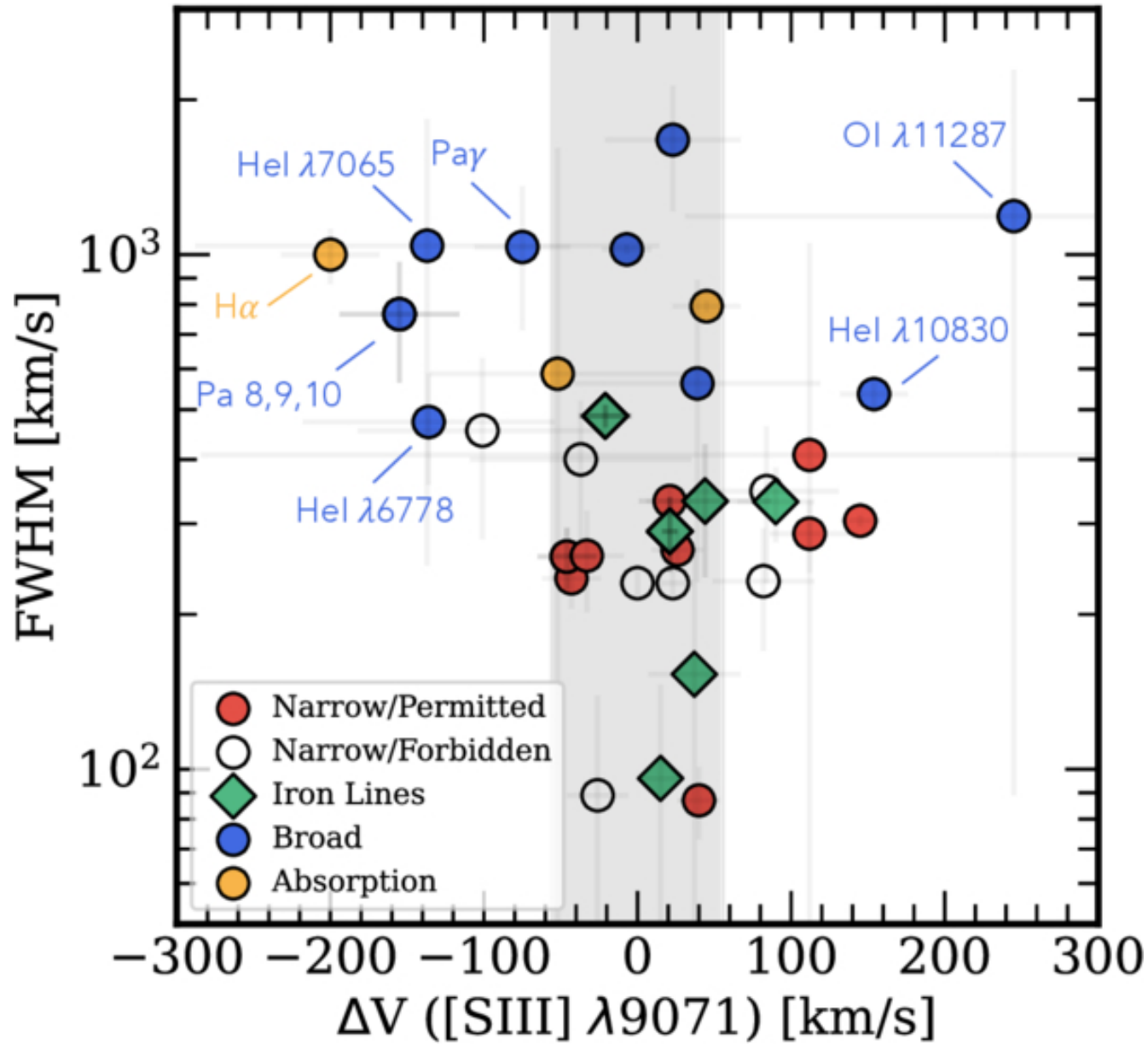
Figure 7. from Vasily Kokorev et al 2026 Astrophys. J. 1004 doi:10.3847/1538-4357/ae4ed7 https://dx.doi.org/10.3847/1538-4357/ae4ed7 © 2026. The Author(s). Published by the American Astronomical Society.
