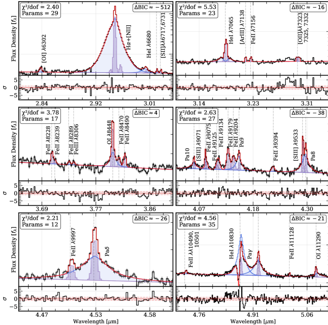
Figure 2. from Vasily Kokorev et al 2026 Astrophys. J. 1004 doi:10.3847/1538-4357/ae4ed7 https://dx.doi.org/10.3847/1538-4357/ae4ed7 © 2026. The Author(s). Published by the American Astronomical Society.
