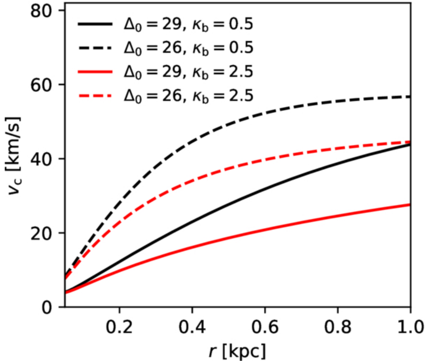
Figure 6. from Yifei Yang and Weikang Lin 2026 Astrophys. J. 1001 doi:10.3847/1538-4357/ae4ed0 https://dx.doi.org/10.3847/1538-4357/ae4ed0 © 2026. The Author(s). Published by the American Astronomical Society.
