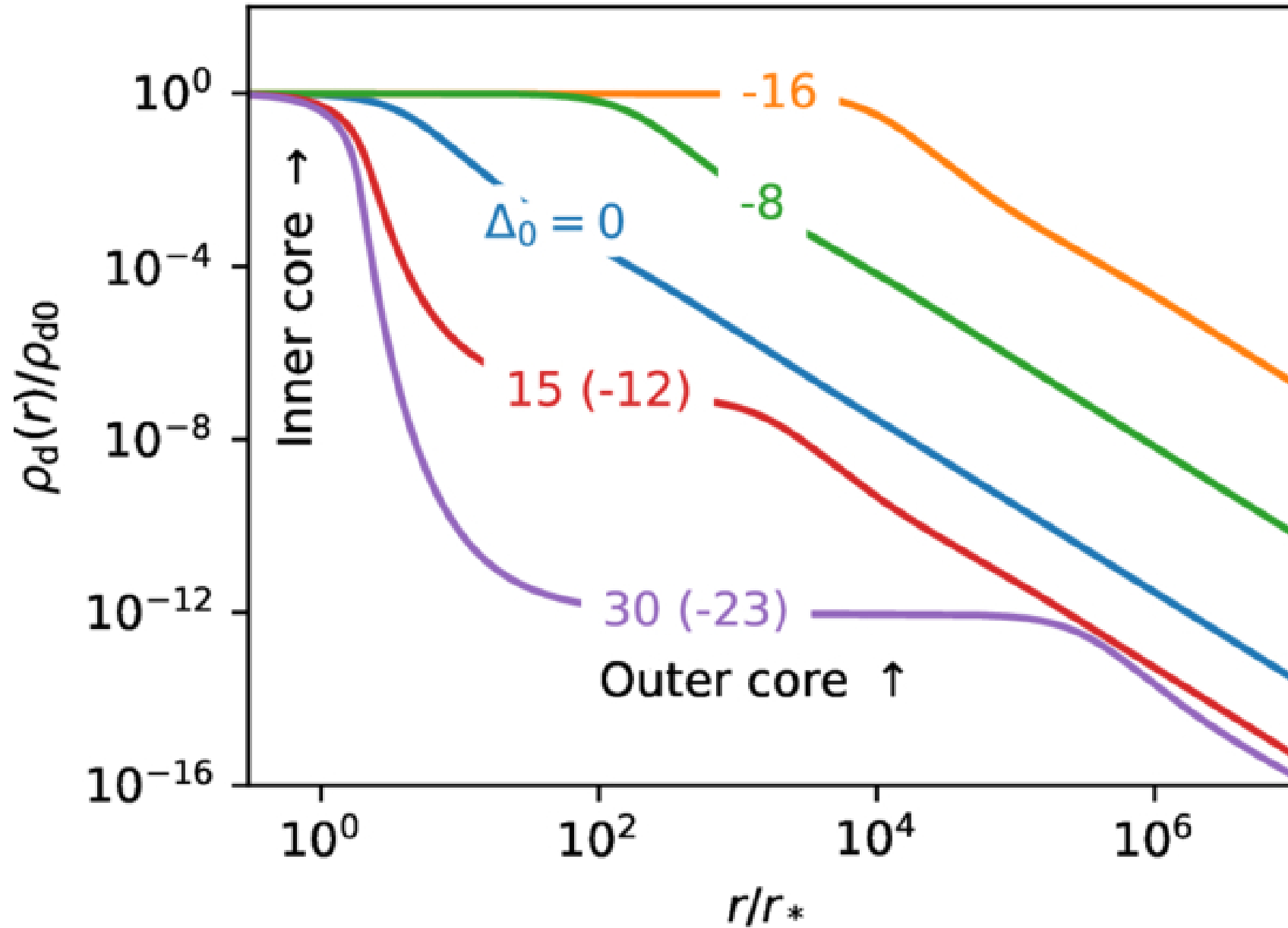
Figure 1. from Yifei Yang and Weikang Lin 2026 Astrophys. J. 1001 doi:10.3847/1538-4357/ae4ed0 https://dx.doi.org/10.3847/1538-4357/ae4ed0 © 2026. The Author(s). Published by the American Astronomical Society.
