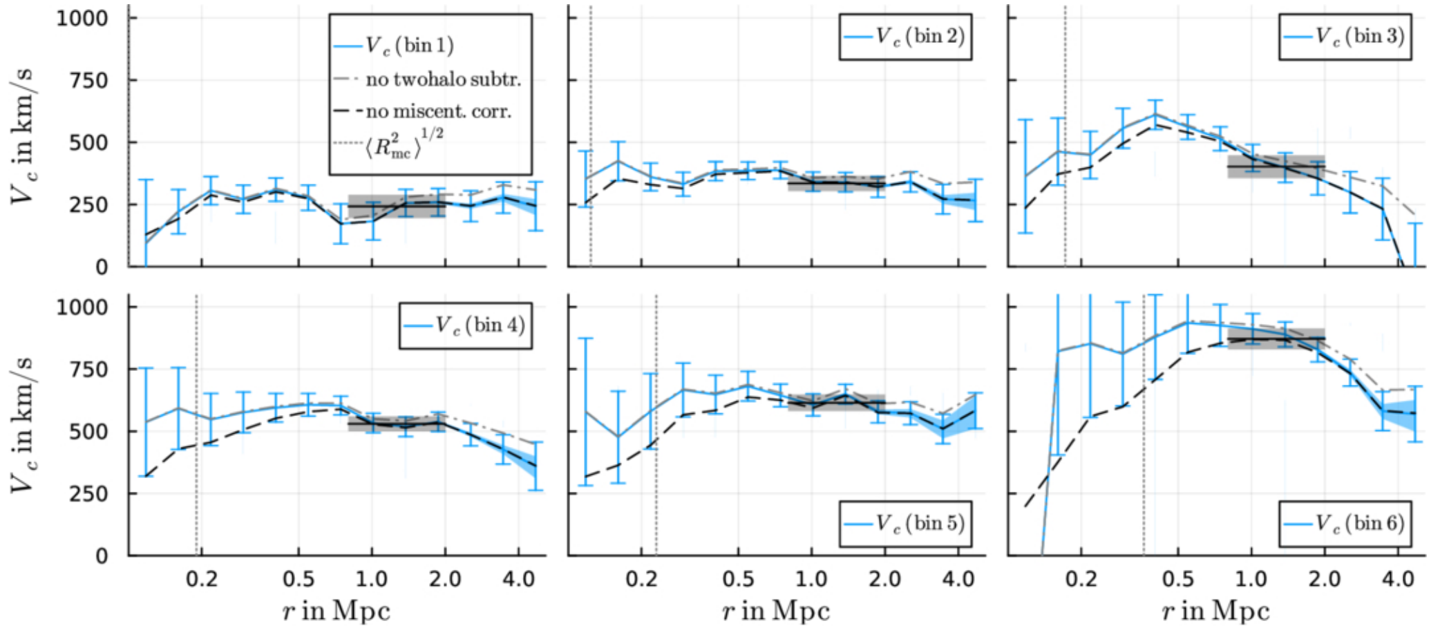
Figure 9. from Stacy S. McGaugh et al 2026 Astrophys. J. 1001 doi:10.3847/1538-4357/ae4ecc https://dx.doi.org/10.3847/1538-4357/ae4ecc © 2026. The Author(s). Published by the American Astronomical Society.
