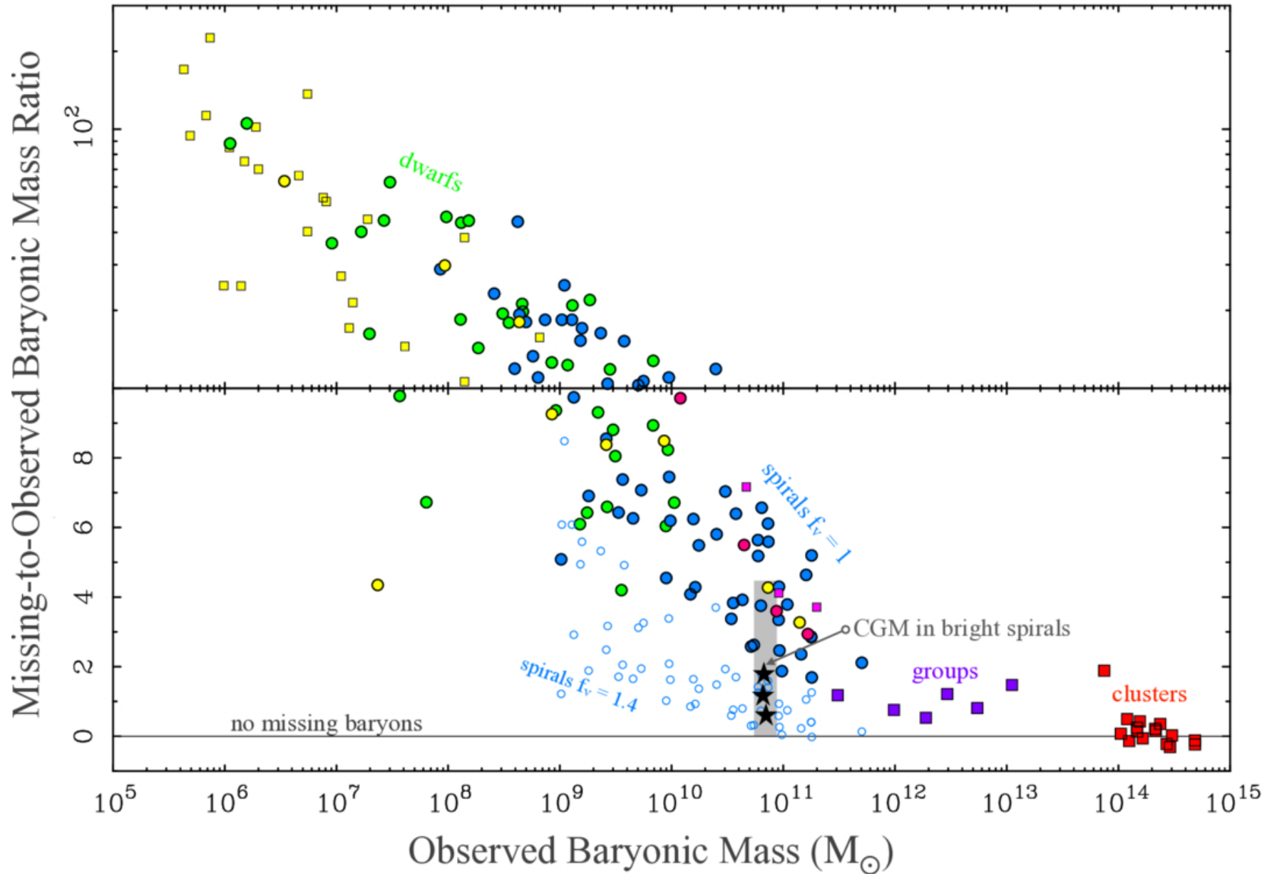
Figure 7. from Stacy S. McGaugh et al 2026 Astrophys. J. 1001 doi:10.3847/1538-4357/ae4ecc https://dx.doi.org/10.3847/1538-4357/ae4ecc © 2026. The Author(s). Published by the American Astronomical Society.
