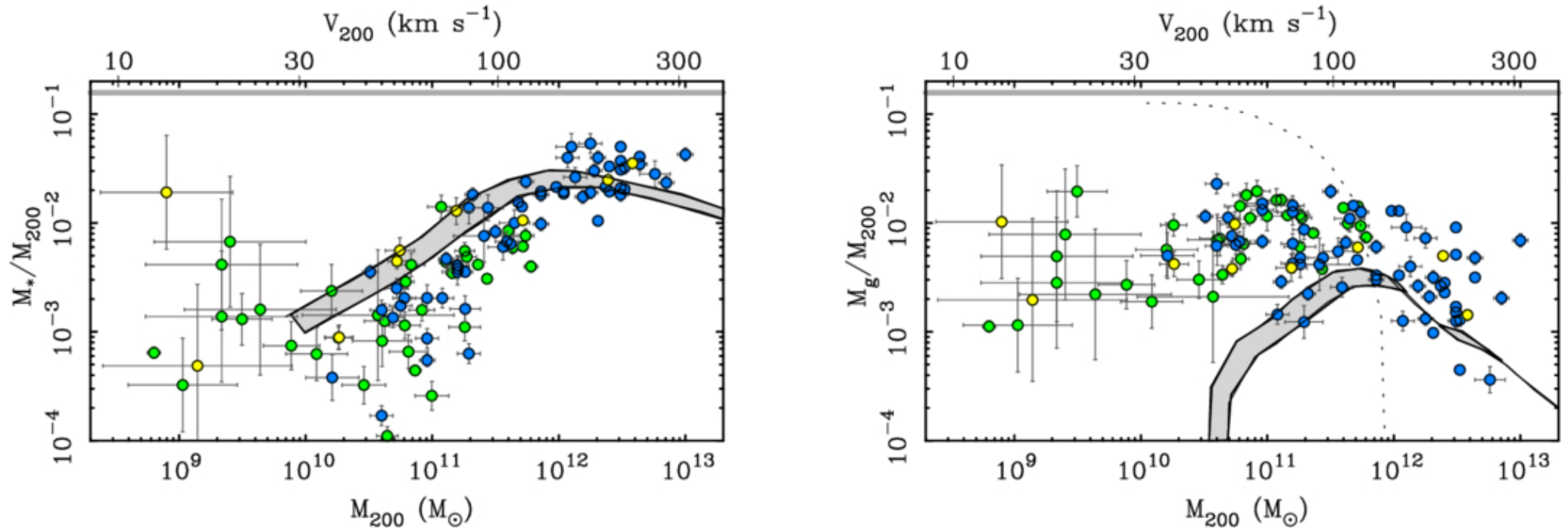
Figure 6. from Stacy S. McGaugh et al 2026 Astrophys. J. 1001 doi:10.3847/1538-4357/ae4ecc https://dx.doi.org/10.3847/1538-4357/ae4ecc © 2026. The Author(s). Published by the American Astronomical Society.
