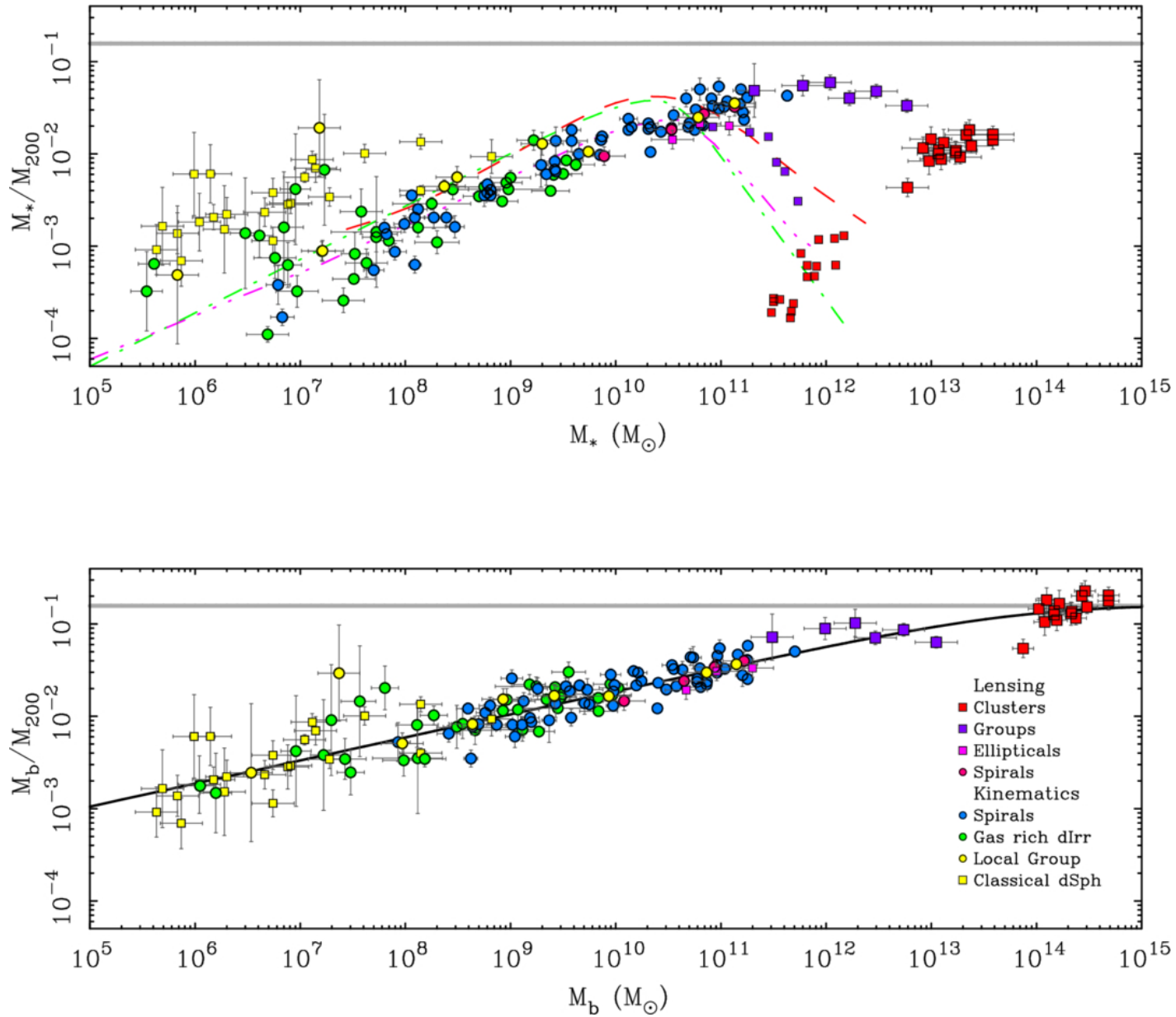
Figure 4. from Stacy S. McGaugh et al 2026 Astrophys. J. 1001 doi:10.3847/1538-4357/ae4ecc https://dx.doi.org/10.3847/1538-4357/ae4ecc © 2026. The Author(s). Published by the American Astronomical Society.
