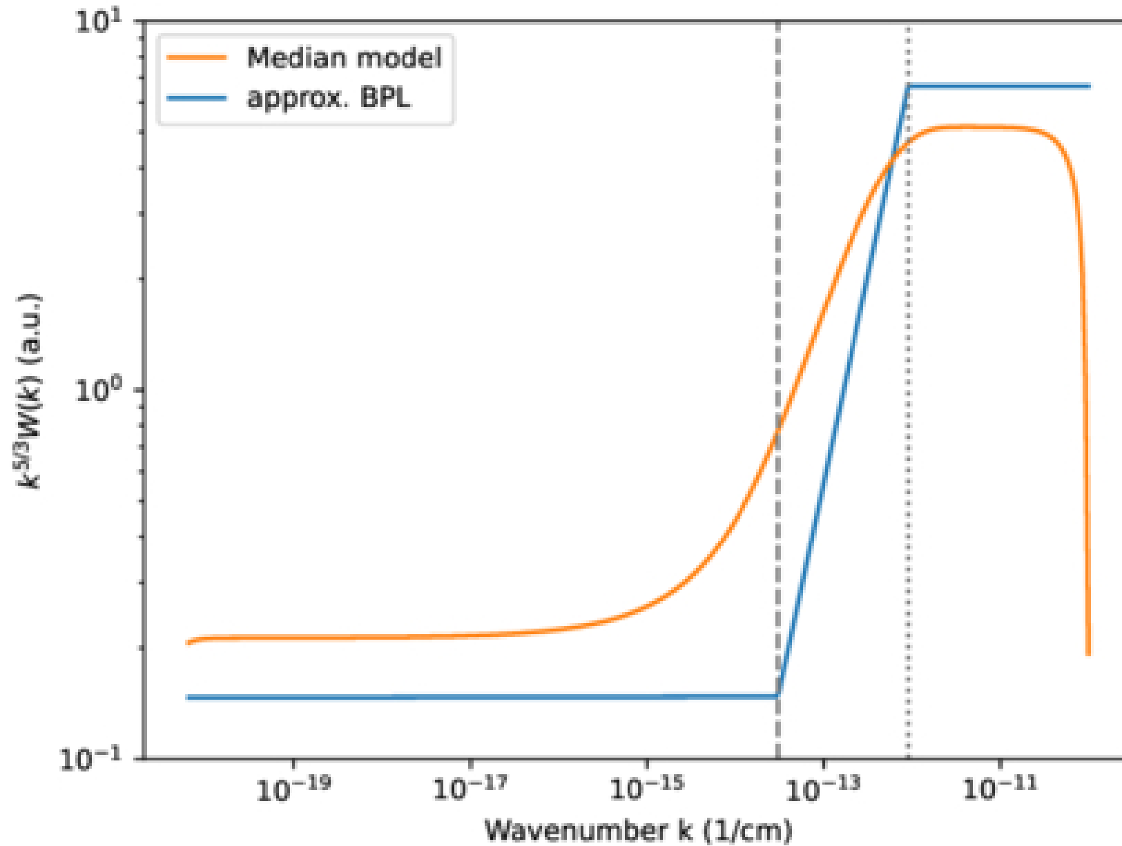
Figure 8. from Linh Han Thanh et al 2026 Astrophys. J. 1001 doi:10.3847/1538-4357/ae4ec4 https://dx.doi.org/10.3847/1538-4357/ae4ec4 © 2026. The Author(s). Published by the American Astronomical Society.
