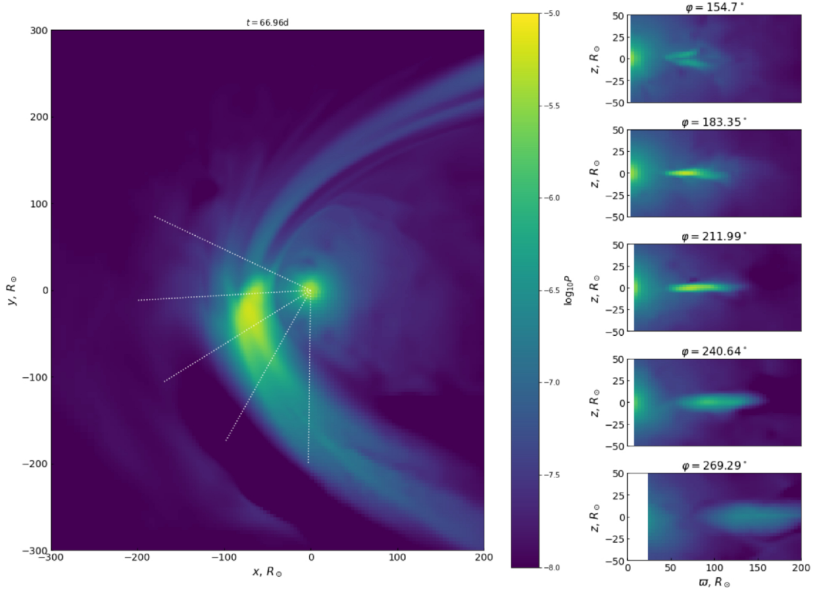
Figure 7. from Pavel Abolmasov et al 2026 Astrophys. J. 1001 doi:10.3847/1538-4357/ae4ebc https://dx.doi.org/10.3847/1538-4357/ae4ebc © 2026. The Author(s). Published by the American Astronomical Society.
