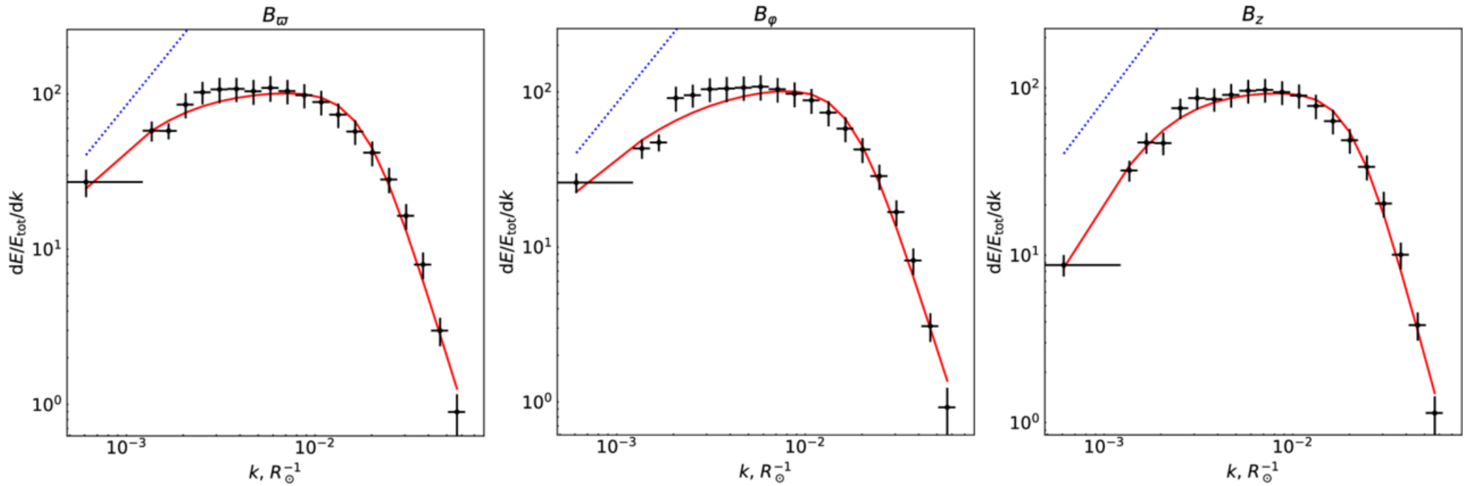
Figure 15. from Pavel Abolmasov et al 2026 Astrophys. J. 1001 doi:10.3847/1538-4357/ae4ebc https://dx.doi.org/10.3847/1538-4357/ae4ebc © 2026. The Author(s). Published by the American Astronomical Society.
