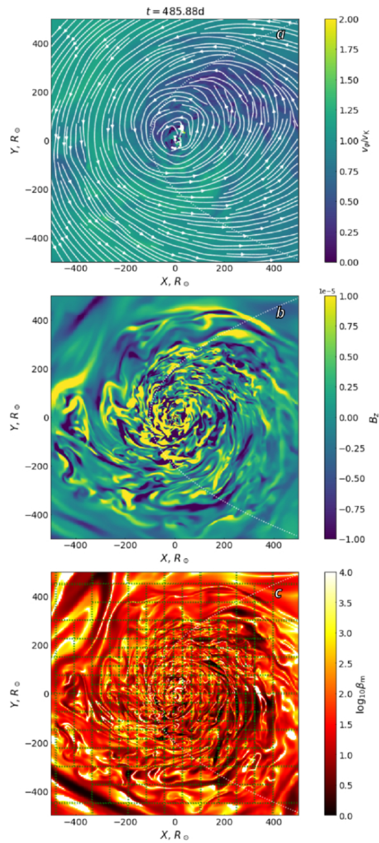
Figure 13. from Pavel Abolmasov et al 2026 Astrophys. J. 1001 doi:10.3847/1538-4357/ae4ebc https://dx.doi.org/10.3847/1538-4357/ae4ebc © 2026. The Author(s). Published by the American Astronomical Society.
