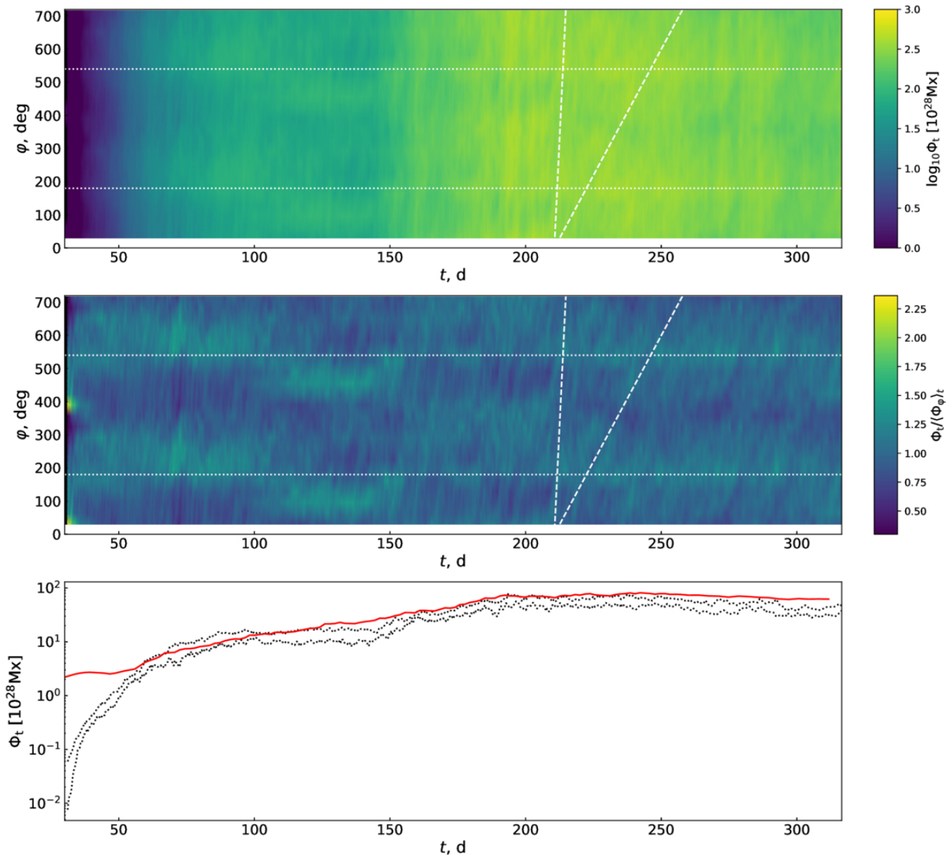
Figure 12. from Pavel Abolmasov et al 2026 Astrophys. J. 1001 doi:10.3847/1538-4357/ae4ebc https://dx.doi.org/10.3847/1538-4357/ae4ebc © 2026. The Author(s). Published by the American Astronomical Society.
