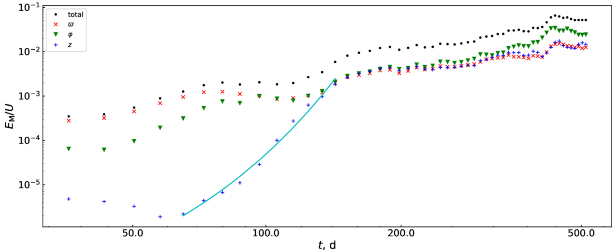
Figure 10. from Pavel Abolmasov et al 2026 Astrophys. J. 1001 doi:10.3847/1538-4357/ae4ebc https://dx.doi.org/10.3847/1538-4357/ae4ebc © 2026. The Author(s). Published by the American Astronomical Society.
