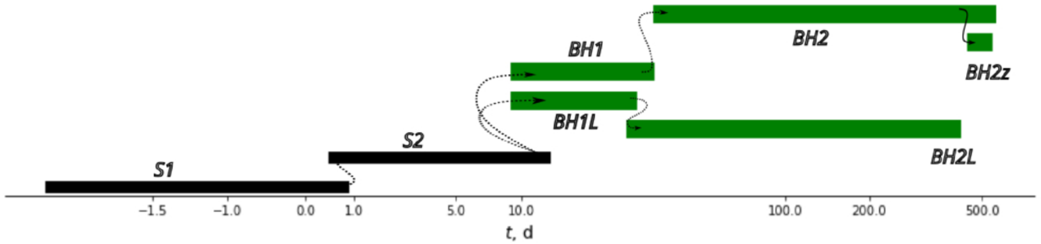
Figure 1. from Pavel Abolmasov et al 2026 Astrophys. J. 1001 doi:10.3847/1538-4357/ae4ebc https://dx.doi.org/10.3847/1538-4357/ae4ebc © 2026. The Author(s). Published by the American Astronomical Society.
