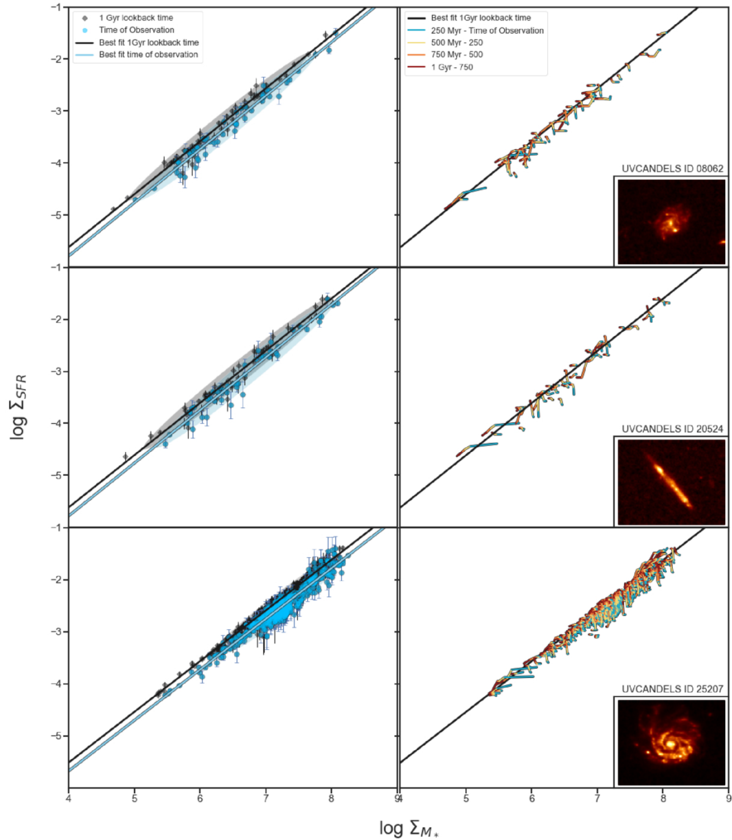
Figure 6. from Charlotte Olsen et al 2026 Astrophys. J. 1001 doi:10.3847/1538-4357/ae4eba https://dx.doi.org/10.3847/1538-4357/ae4eba © 2026. The Author(s). Published by the American Astronomical Society.
