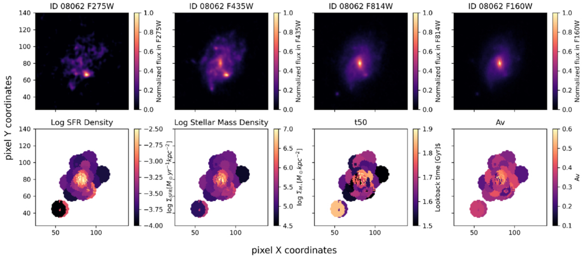
Figure 3. from Charlotte Olsen et al 2026 Astrophys. J. 1001 doi:10.3847/1538-4357/ae4eba https://dx.doi.org/10.3847/1538-4357/ae4eba © 2026. The Author(s). Published by the American Astronomical Society.
