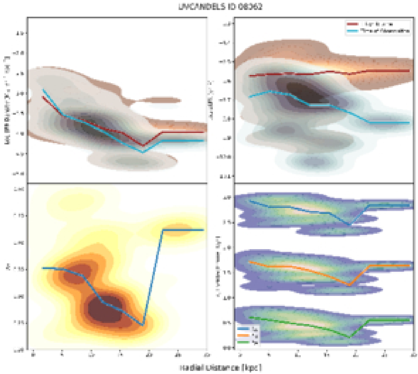
Figure 20. from Charlotte Olsen et al 2026 Astrophys. J. 1001 doi:10.3847/1538-4357/ae4eba https://dx.doi.org/10.3847/1538-4357/ae4eba © 2026. The Author(s). Published by the American Astronomical Society.
