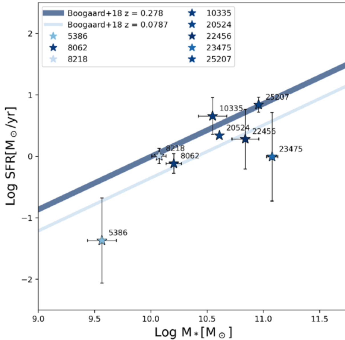
Figure 2. from Charlotte Olsen et al 2026 Astrophys. J. 1001 doi:10.3847/1538-4357/ae4eba https://dx.doi.org/10.3847/1538-4357/ae4eba © 2026. The Author(s). Published by the American Astronomical Society.
