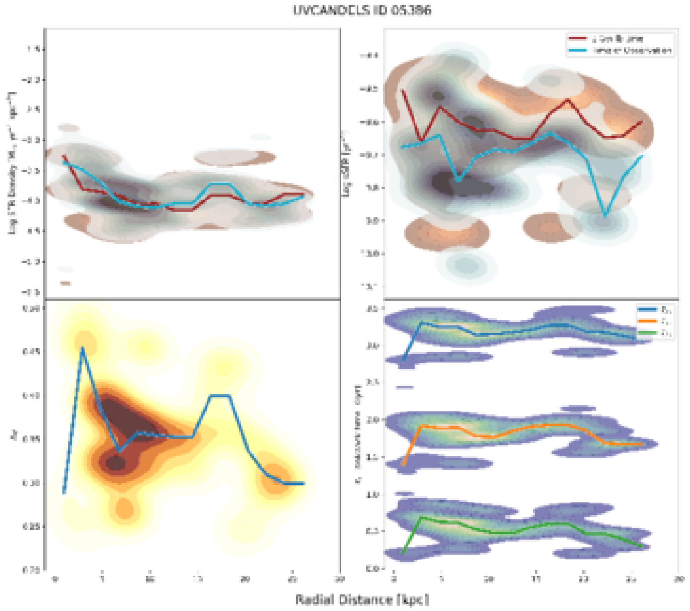
Figure 19. from Charlotte Olsen et al 2026 Astrophys. J. 1001 doi:10.3847/1538-4357/ae4eba https://dx.doi.org/10.3847/1538-4357/ae4eba © 2026. The Author(s). Published by the American Astronomical Society.
