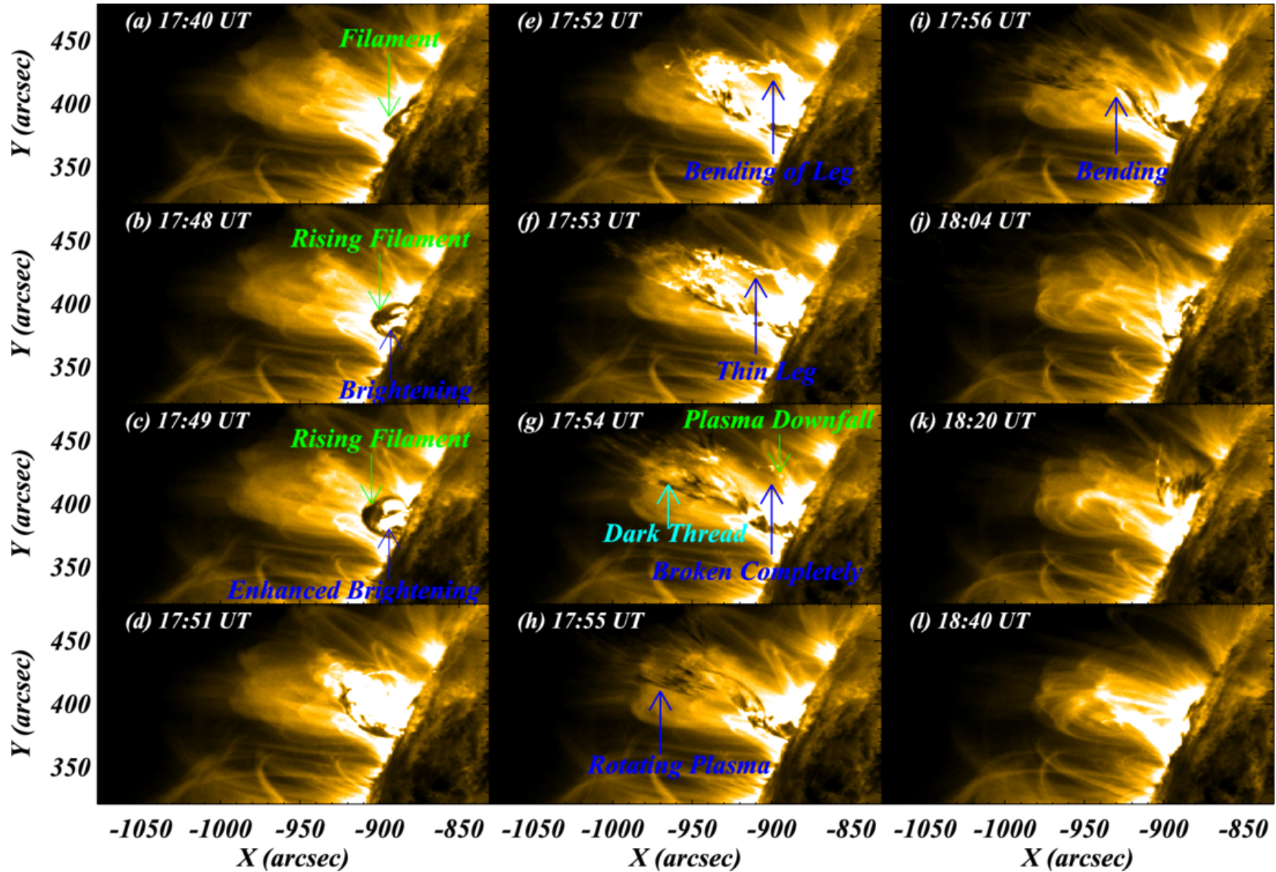
Figure 4. from Pradeep Kayshap et al 2026 Astrophys. J. 1001 doi:10.3847/1538-4357/ae4e2c https://dx.doi.org/10.3847/1538-4357/ae4e2c © 2026. The Author(s). Published by the American Astronomical Society.
