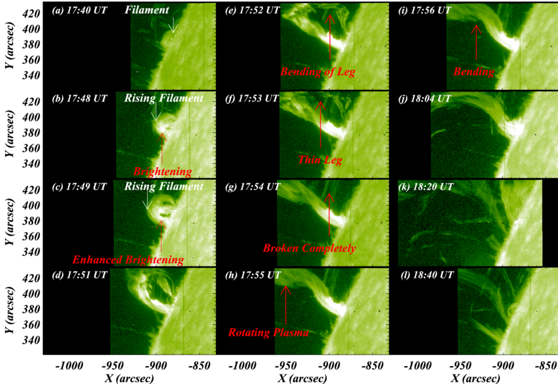
Figure 3. from Pradeep Kayshap et al 2026 Astrophys. J. 1001 doi:10.3847/1538-4357/ae4e2c https://dx.doi.org/10.3847/1538-4357/ae4e2c © 2026. The Author(s). Published by the American Astronomical Society.
