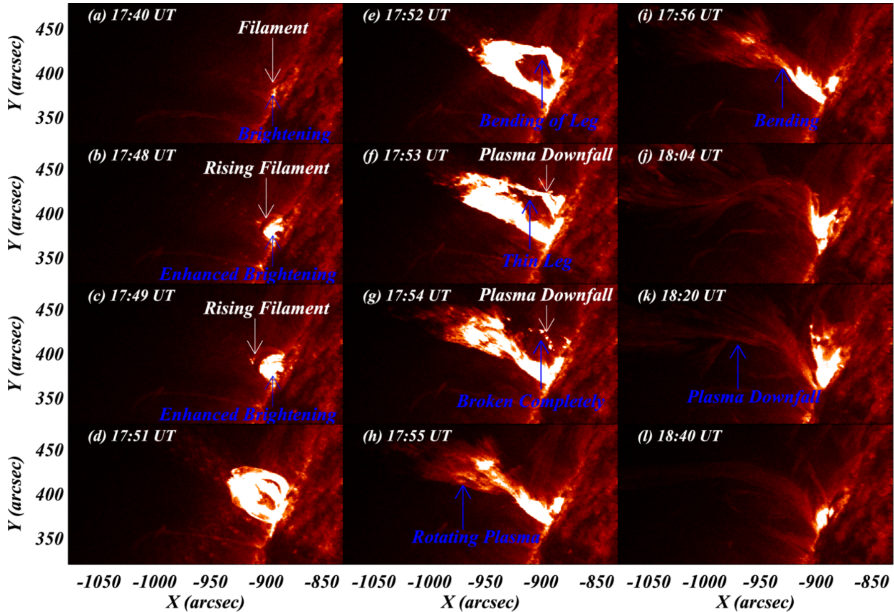
Figure 2. from Pradeep Kayshap et al 2026 Astrophys. J. 1001 doi:10.3847/1538-4357/ae4e2c https://dx.doi.org/10.3847/1538-4357/ae4e2c © 2026. The Author(s). Published by the American Astronomical Society.
