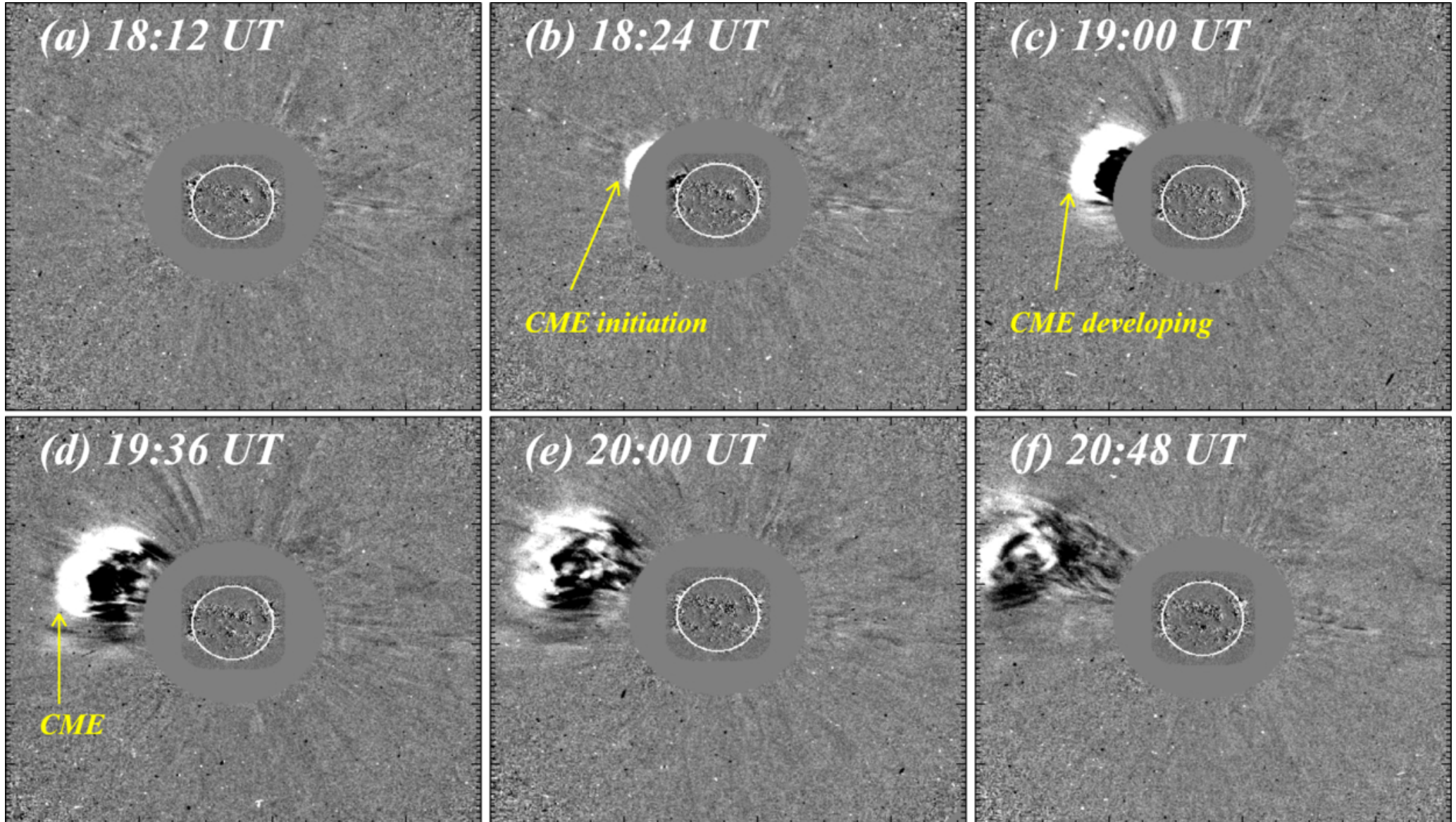
Figure 11. from Pradeep Kayshap et al 2026 Astrophys. J. 1001 doi:10.3847/1538-4357/ae4e2c https://dx.doi.org/10.3847/1538-4357/ae4e2c © 2026. The Author(s). Published by the American Astronomical Society.
