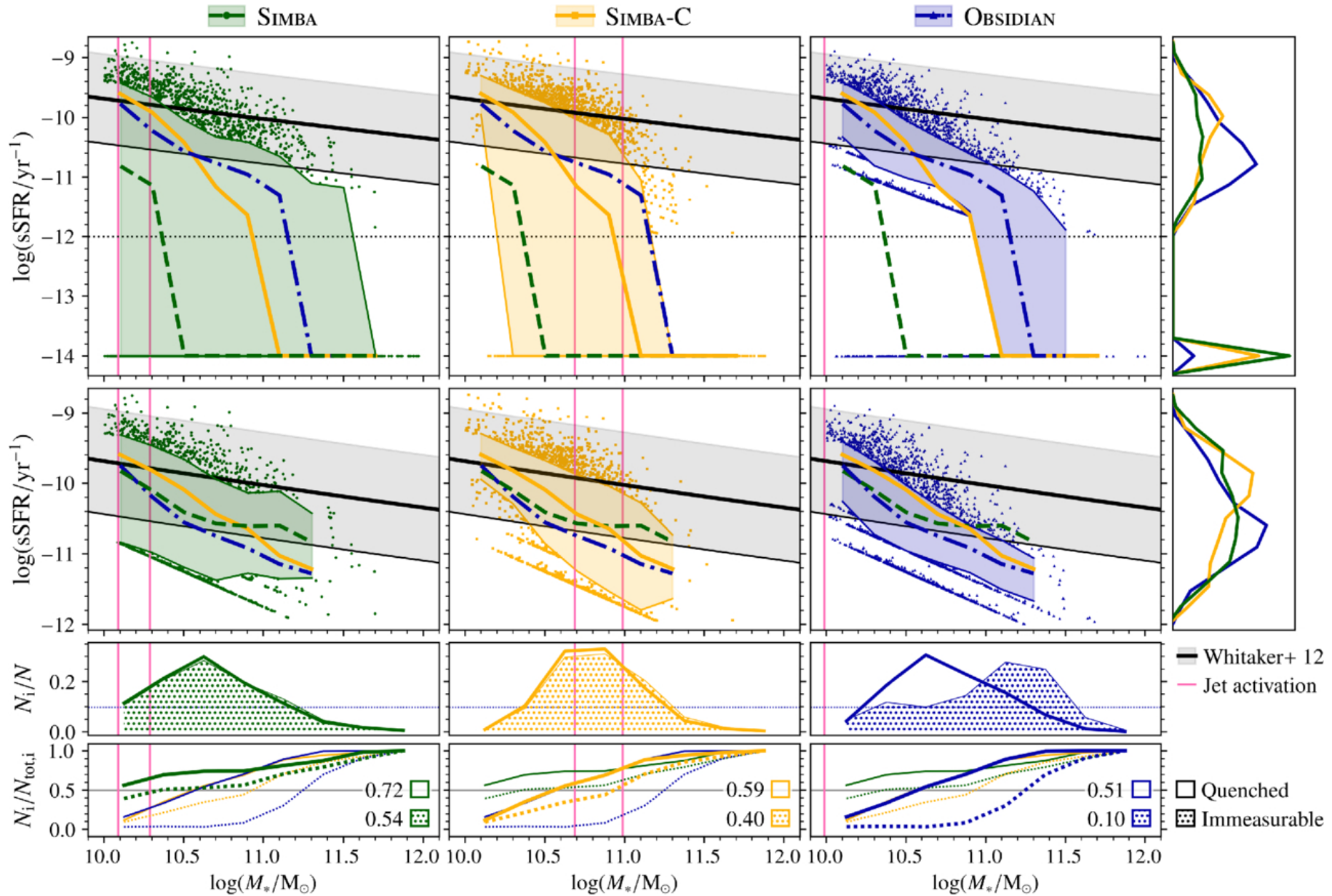
Figure 9. from Ruxin Barré et al 2026 Astrophys. J. 1001 doi:10.3847/1538-4357/ae4e2a https://dx.doi.org/10.3847/1538-4357/ae4e2a © 2026. The Author(s). Published by the American Astronomical Society.
