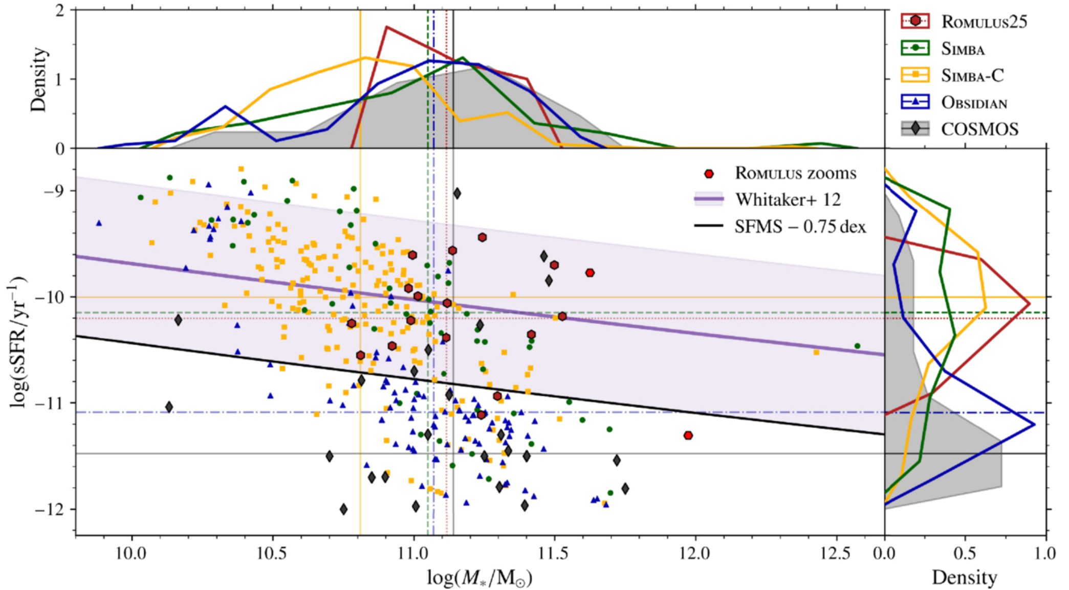
Figure 6. from Ruxin Barré et al 2026 Astrophys. J. 1001 doi:10.3847/1538-4357/ae4e2a https://dx.doi.org/10.3847/1538-4357/ae4e2a © 2026. The Author(s). Published by the American Astronomical Society.
