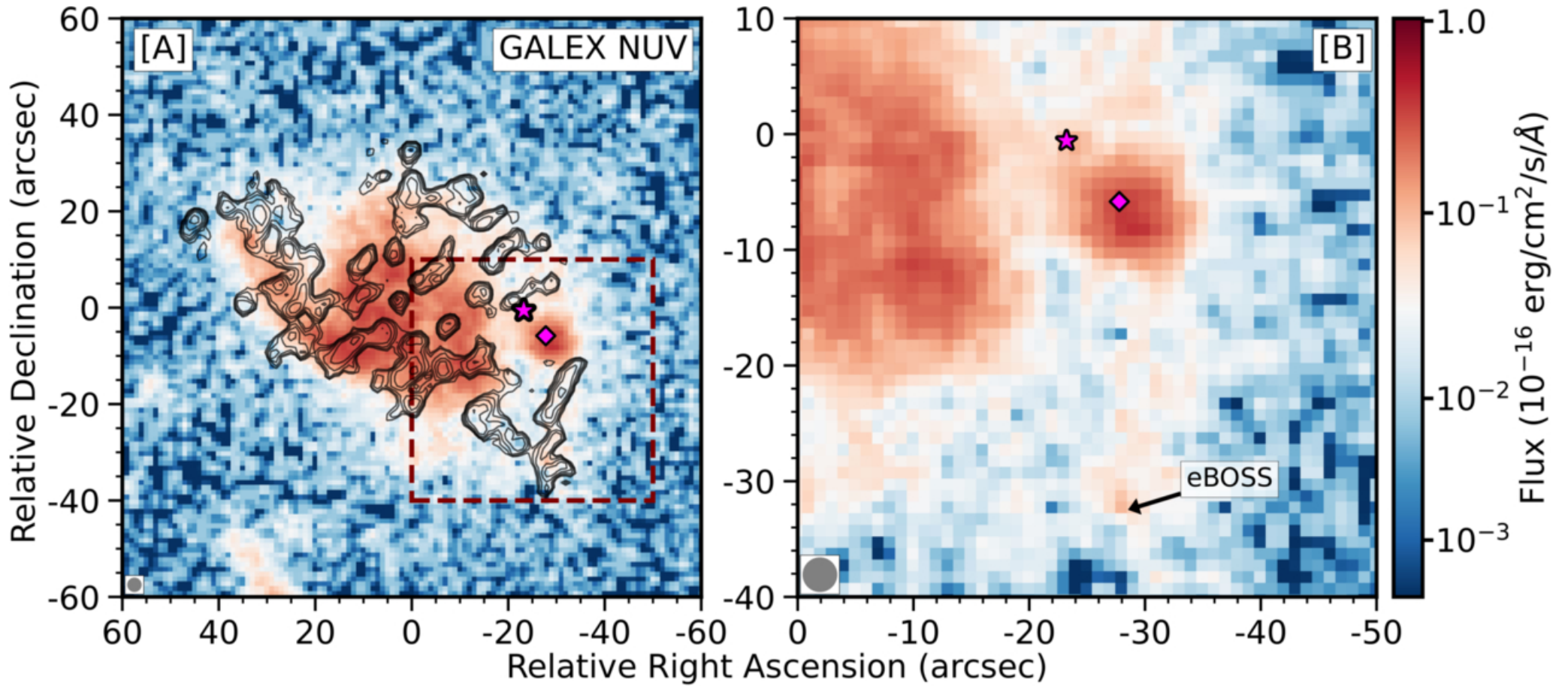
Figure 5. from Balpreet Kaur et al 2026 Astrophys. J. 1001 doi:10.3847/1538-4357/ae4d4a https://dx.doi.org/10.3847/1538-4357/ae4d4a © 2026. The Author(s). Published by the American Astronomical Society.
