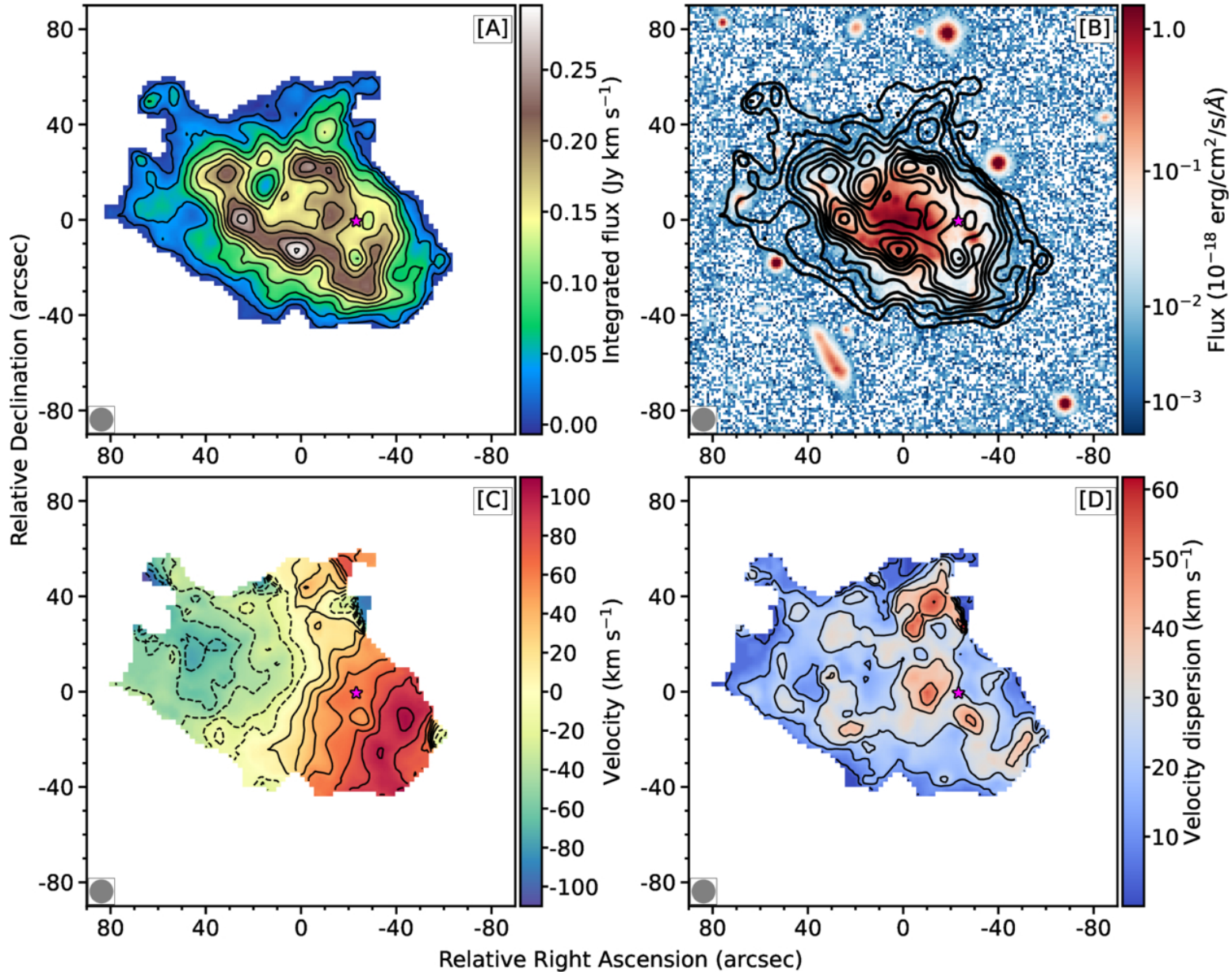
Figure 3. from Balpreet Kaur et al 2026 Astrophys. J. 1001 doi:10.3847/1538-4357/ae4d4a https://dx.doi.org/10.3847/1538-4357/ae4d4a © 2026. The Author(s). Published by the American Astronomical Society.
