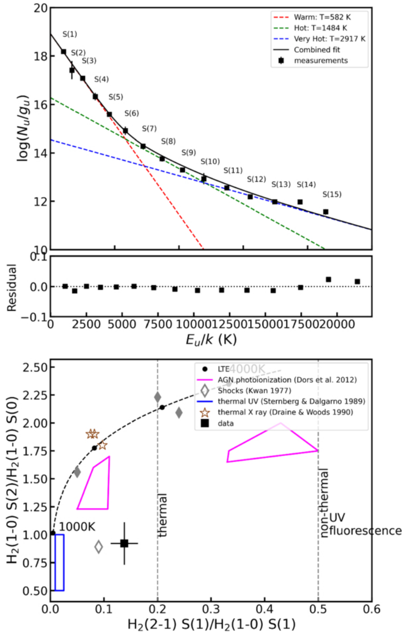
Figure 5. from Payel Nandi et al 2026 Astrophys. J. 1001 doi:10.3847/1538-4357/ae4d1a https://dx.doi.org/10.3847/1538-4357/ae4d1a © 2026. The Author(s). Published by the American Astronomical Society.
