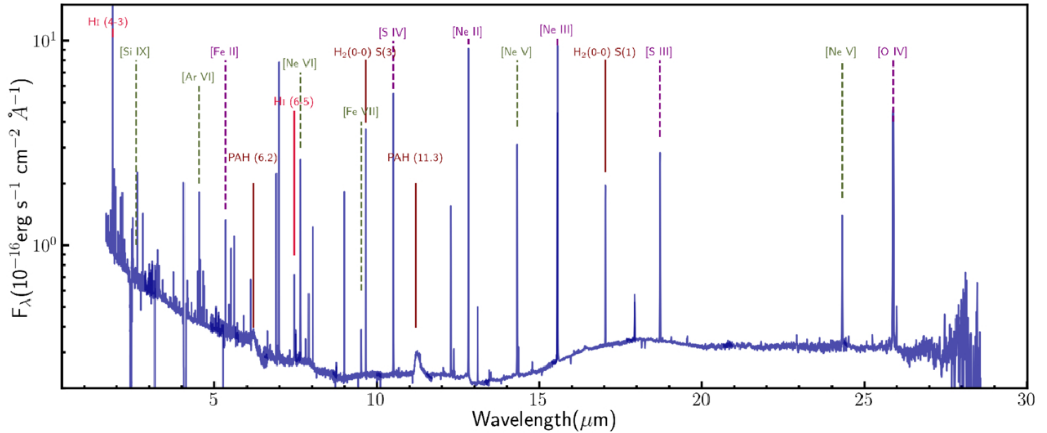
Figure 1. from Payel Nandi et al 2026 Astrophys. J. 1001 doi:10.3847/1538-4357/ae4d1a https://dx.doi.org/10.3847/1538-4357/ae4d1a © 2026. The Author(s). Published by the American Astronomical Society.
