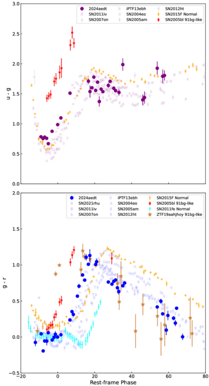
Figure 9. from Dezheng Meng et al 2026 Astrophys. J. 1002 doi:10.3847/1538-4357/ae4c87 https://dx.doi.org/10.3847/1538-4357/ae4c87 © 2026. The Author(s). Published by the American Astronomical Society.
