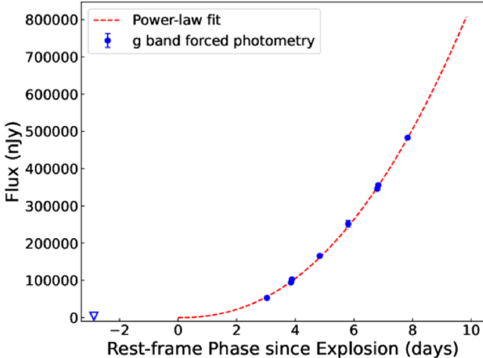
Figure 5. from Dezheng Meng et al 2026 Astrophys. J. 1002 doi:10.3847/1538-4357/ae4c87 https://dx.doi.org/10.3847/1538-4357/ae4c87 © 2026. The Author(s). Published by the American Astronomical Society.
