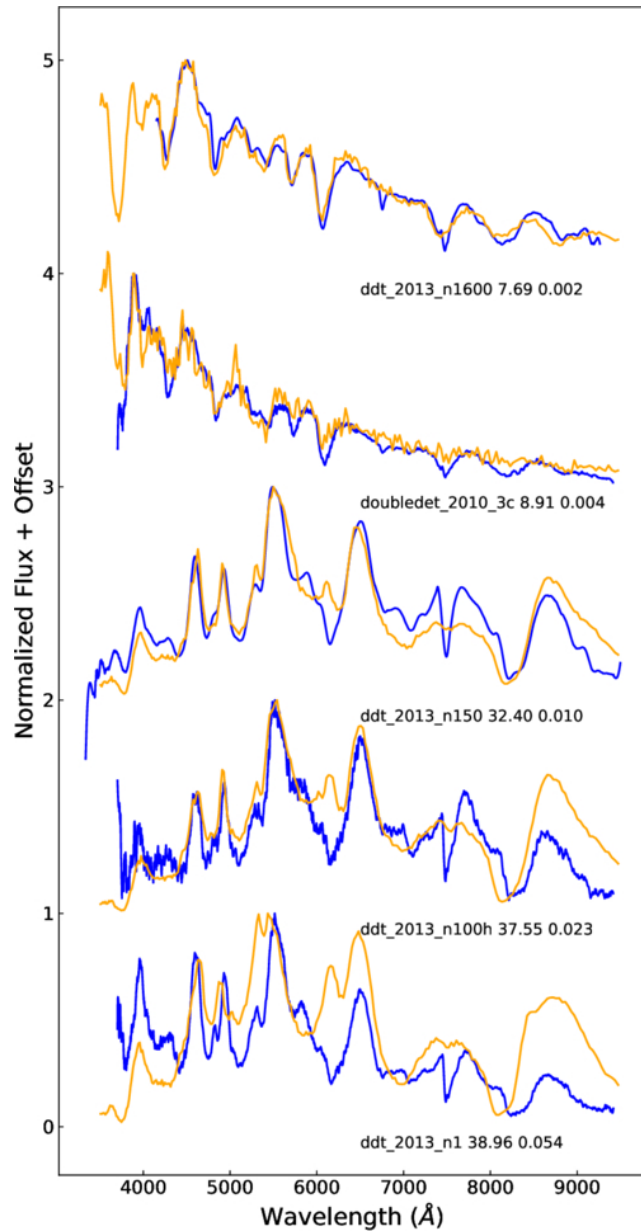
Figure 19. from Dezheng Meng et al 2026 Astrophys. J. 1002 doi:10.3847/1538-4357/ae4c87 https://dx.doi.org/10.3847/1538-4357/ae4c87 © 2026. The Author(s). Published by the American Astronomical Society.
